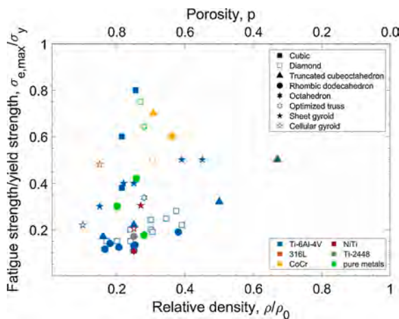
Fig. 15. Compression-compression fatigue strength normalized with respect to the yield strength as a function of the open porosity, p . \sigma_{e,max} is the fatigue strength at 10^6 cycles to failure corresponding to the maximum compressive global stress applied to the sample. The data were taken from [103–119]. Where available, the measured porosity is used instead of the as-designed one. Fatigue experiments were carried out in air at load ratio R = 0.1 . The vertical arrow indicates no failure for cubic cells tested at maximum stress up to 80 % of the yield strength.
