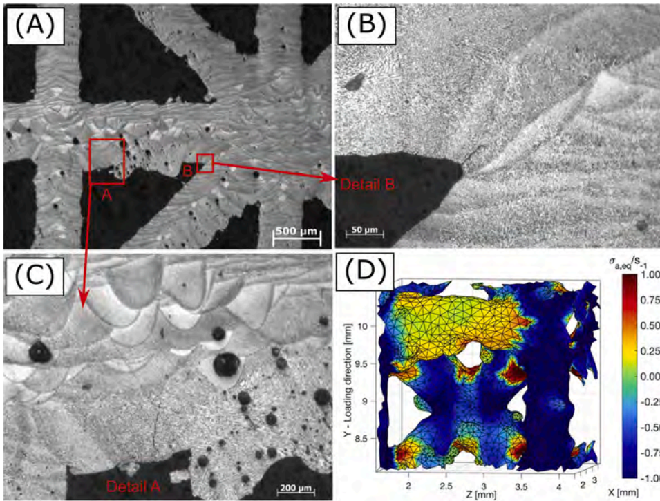
Fig. 27. Fatigue cracks in FCC lattices made of AlSi 7 Mg [123]. (A), (B), (C) Optical micrograph showing crack initiation in a horizontal strut at a geometrical imperfection located in the vicinity of the node. (D) stress distribution estimated from FEM simulations of the real lattice geometry reconstructed via CT scans. Hot spots (red coloured regions) are located in the vicinity of lattice nodes. (For interpretation of the references to colour in this figure legend, the reader is referred to the web version of this article).
