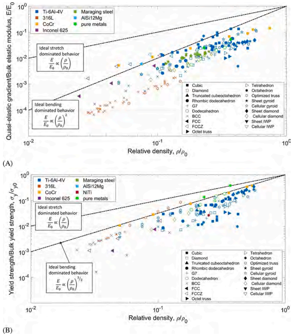
Fig. 9. Relative quasi elastic gradient (A) and relative yield strength (B) as a function of relative density for cellular lattice materials investigated in the literature [38,49,56,57,66–87] with various unit cell architecture.
