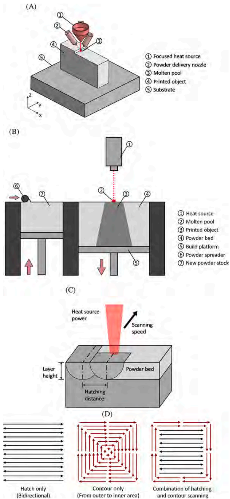
Fig. 4. Schematic illustration of (A) DED [44] and (B) PBF processes; (C) process parameters in PBF [45]; (D) various scanning strategies.
