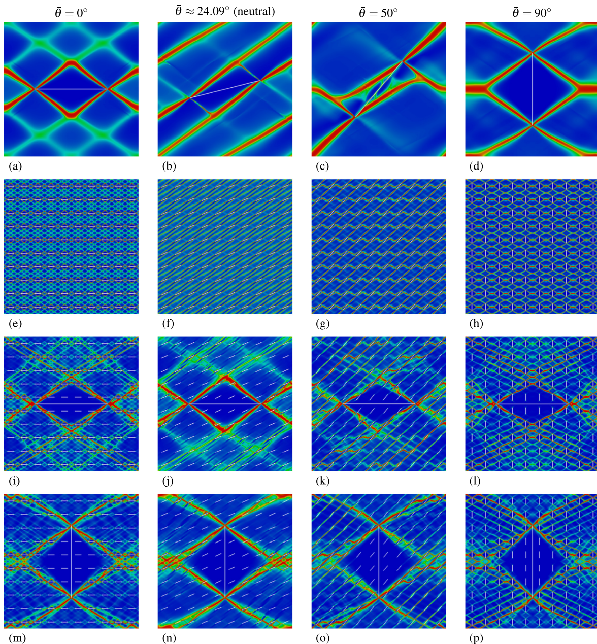
Fig. 19. Maps of damage field \omega revealing shear band patterns in a unit square cell (of side L ) subject to macroscopic straining in the vertical direction and containing different RLIs’ distributions. Upper row: one large (or ‘macro’) RLI ( a = L/4 ); Second row: a periodic distribution of small (or ‘micro’) RLIs ( a = L/40 ); Third row: one large horizontal RLI inside a periodic distribution of small RLIs at different inclinations ( \bar{\theta} = \{0, 24.09, 50, 90\}^\circ ); Lower row: as in the third row, but the large RLI is vertical. The color scale is the same as in Fig. 9.
