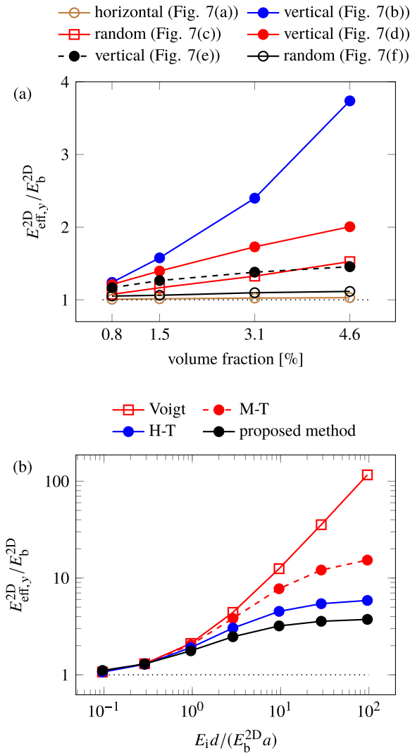
Fig. 8. Predicted effective Young's modulus E_{\text{eff},y}^{2D} of a composite (a) with an increasing number of RLLs for distributions similar to those shown in Fig. 7 and (b) for 1500 vertical inclusions (oriented along the y axis, Fig. 7(b)) as a function of the ratio E_i d / (E_b^{2D} a) . Analytical micromechanical estimates (Voigt, Halpin-Tsai (H-T), and Mori-Tanaka (M-T)) are also included.
