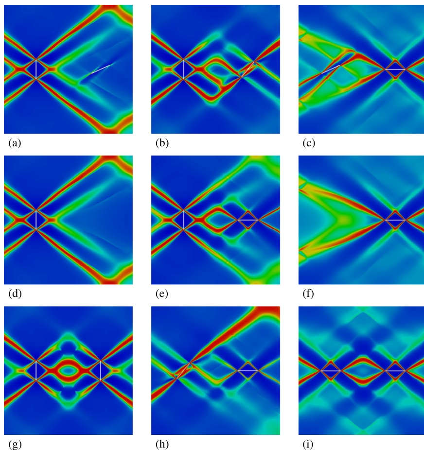
Fig. 11. Localization of damage \omega showing shear bands originating from the interaction of two RLI at various inclinations: (a) vertical ( \bar{\theta} = 90^\circ ) and at neutral inclination ( \bar{\theta} = \bar{\theta}_n \approx 24.09^\circ ), (b) vertical ( \bar{\theta} = 90^\circ ) and inclined at \bar{\theta} = 50^\circ , (c) neutral ( \bar{\theta} = \bar{\theta}_n \approx 24.09^\circ ) and horizontal ( \bar{\theta} = 0^\circ ), (d) only one vertical inclusion is considered, (e) vertical and horizontal, (f) only one horizontal inclusion is considered, (g) both vertical, (h) inclined at \bar{\theta} = 50^\circ and horizontal, (i) both horizontal. The two cases in panels (d) and (f) with only one inclusion have been included for comparison purposes. The color scale is the same as in Fig. 9.
