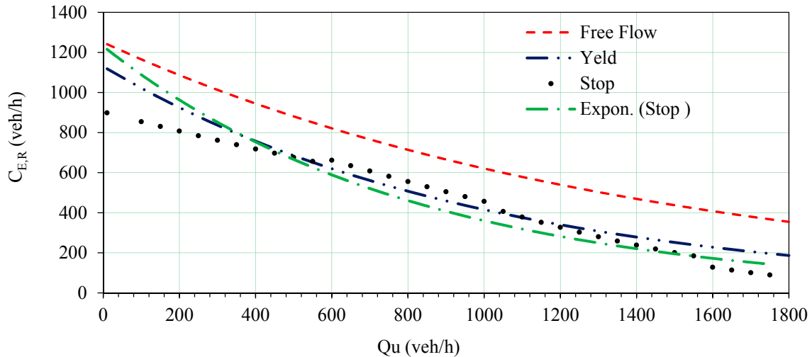
Figure 5. Bypass capacity laws (source: [15]).
