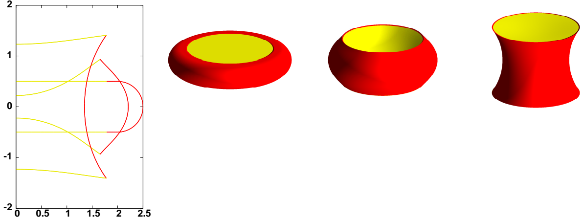
Figure 5: ( C^0 with phase area and volume conservation) Plots at times t = 0, 0.1, 1 .
