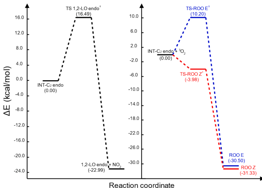
Fig. 10. PES at the CCSD(T)/CBS level with ZPE correction at the UB3LYP/6-31+G(d,p) level of epoxide formation (left) and molecular oxygen addition (right).
