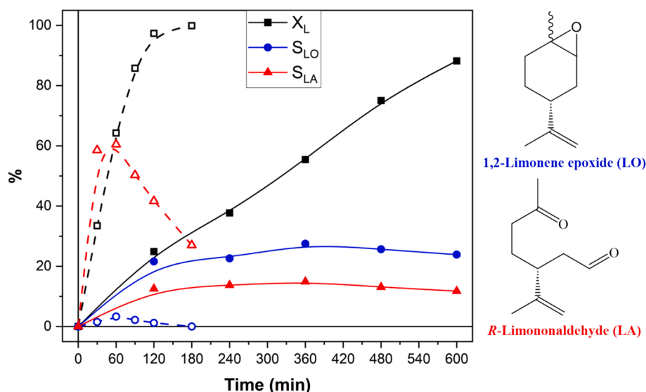
Fig. 5. R-Limonene conversion ( X_L ; black squares), selectivity towards 1,2-limonene epoxide (LO) ( S_{LO} ; blue circles), selectivity towards R-limononanaldehyde (LA) ( S_{LA} ; red triangles). Reaction conditions for solid line trends: R-limonene 2 mM, \text{LiNO}_3 10 mM, Ag-TiO 2 0.5 g/L in acetonitrile. Reaction conditions for dashed line trends: R-limonene 2 mM, AgNO 3 10 mM, bare TiO 2 0.5 g/L in acetonitrile.
