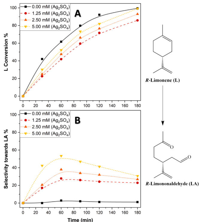
Fig. 1. R -Limonene (L) conversion (Panel A) and selectivity towards R -limononaldehyde (LA) (Panel B) at constant amount of bare \text{TiO}_2 (0.5 g/L) and \text{LiNO}_3 (10 mM), by varying the concentration of \text{Ag}_2\text{SO}_4 , i.e. 0 mM (black squares), 1.25 mM (red circles), 2.5 mM (orange upward triangles), 5.0 mM (yellow downward triangles).
