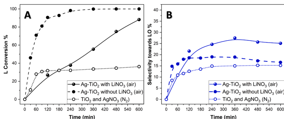
Fig. 6. Conversion of R-limonene (L) (Panel A, black curves) and selectivity towards 1,2-limonene epoxide (LO) (Panel B, blue curves) under different reaction conditions: Solid line trends: R-limonene 2 mM, \text{LiNO}_3 10 mM, Ag-TiO 2 0.5 g/L under static air in acetonitrile. Dashed line trends: R-limonene 2 mM, Ag-TiO 2 0.5 g/L under static air in acetonitrile. Dotted line trends: R-limonene 2 mM, AgNO 3 10 mM, TiO 2 0.5 g/L under \text{N}_2 in acetonitrile.
