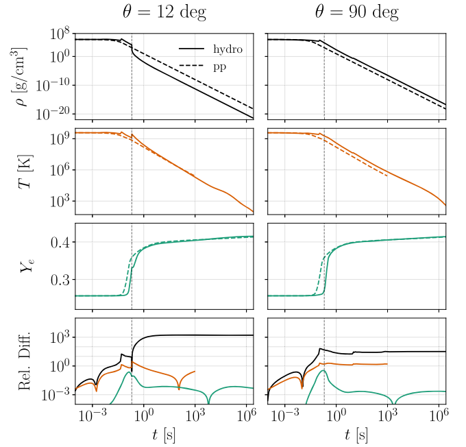
Figure 5. Evolution of the density (black), temperature (orange), and electron fraction (green) in the innermost shell of the 12^\circ (left column) and 90^\circ (right column) angular sections of the ejecta as calculated from the complete simulation (solid lines) and an independent SkyNet run (dashed lines). The bottom panels show the relative differences calculated with an expression analogous to Equation (5). The evolution of the temperature from SkyNet is plotted until it is actively updated by the NN and used in the nuclear calculations. The vertical dashed line at t = 200 ms indicates the launch of the jet.
