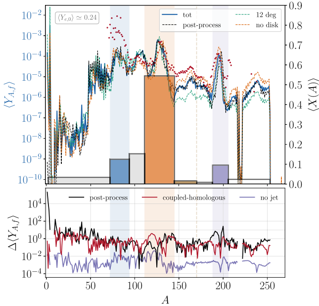
Figure 2. Global r -process nucleosynthesis yields at t \simeq 5 \times 10^4 s. Top panel: in blue and black, the final global abundances \langle Y_{A,f} \rangle as a function of the mass number A , obtained, respectively, from our SNEC simulation and with a postprocess analysis similar to A. Perego et al. (2022). In orange and green are the results obtained from our SNEC simulation excluding the disk ejecta or including only the matter emitted at \theta = 12^\circ (at all times). Red dots represent the solar r -abundances (N. Prantzos et al. 2020) scaled to match the average value of the second peak. The histogram shows, for the complete simulation, the global cumulative mass fractions \langle X(A) \rangle of selected groups of elements, in particular, first (blue), second (orange), and third (purple) r -process peaks and rare earths (brown). We report the initial value of the average electron fraction of the ejecta in the top left corner of the plot. Bottom panel: in red, the relative difference against the model with prescribed homologous expansion (see Equation (5)), and in black and purple, analogous comparisons between our global results and the postprocess analysis and between the results of the complete simulation with and without the jet. The differences are only shown for mass numbers \hat{A} such that \langle Y_{\hat{A},f} \rangle > 10^{-10} .
