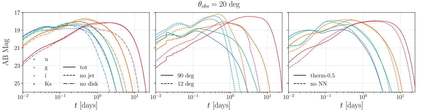
Figure 4. AB apparent magnitudes predicted by our simulation for the Gemini bands u , g , i , and K s for an observation angle of \theta = 20^\circ and a distance of 40 Mpc. Left panel: results of the complete simulation (solid lines) against the predictions obtained by excluding the jet (dashed lines) or the disk component (dashed-dotted lines). Central panel: isotropized \theta = 12^\circ, 90^\circ angular sections (solid and dashed lines, respectively). Right panel: light curves obtained assuming a constant thermalization factor f_{th} = 0.5 with (solid lines) or without (with the same heating rate fits of Z. Wu et al. 2022; dashed lines) a coupled NN.
