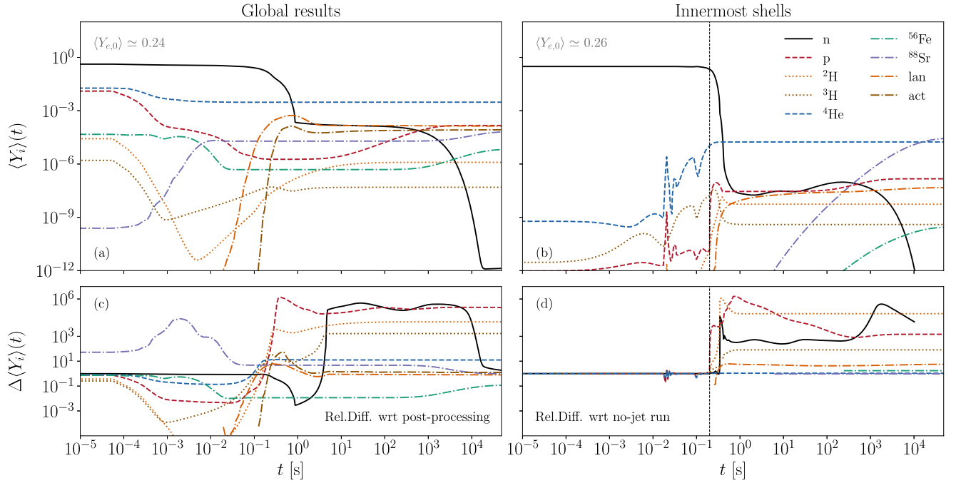
Figure 3. Evolution of the abundances of a few selected isotopes and the cumulative abundances of lanthanides and actinides. Panel (a) shows global results obtained with mass-weighted averages all over the ejecta. Panel (b) is restricted to an average over the innermost shell of all the angular sections in order to highlight the jet effects. Panel (c) shows the ratio \Delta \langle Y_i \rangle = \langle Y_i \rangle / \langle Y_i^{pp} \rangle between our results and the prediction obtained with a postprocess procedure similar to the one of A. Perego et al. (2022); see Appendix C for details. Panel (d) shows a similar comparison between the results obtained with and without the jet. The vertical dashed lines in panels (b) and (d) indicate the time when the jet is launched. In panels (c) and (d), the results are only shown for times t such that \langle Y_i \rangle(t) > 10^{-12} .
