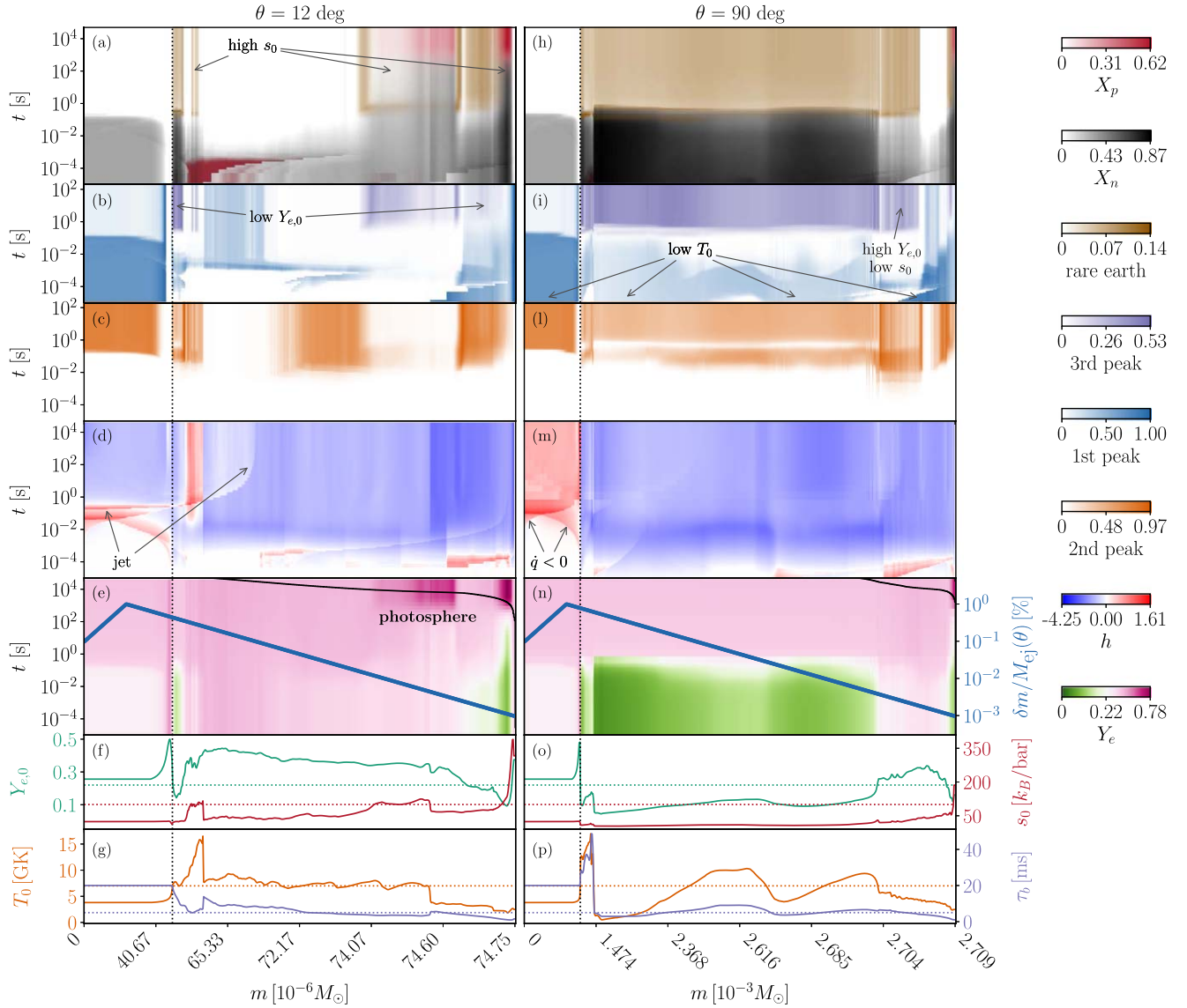
Figure 1. Evolution of the ejecta composition for every mass shell of the angular sections \theta \simeq 12^\circ, 90^\circ (first and second column, respectively). The x-axis indicates the Lagrangian mass coordinate, linear in the shell index. The vertical black dotted lines indicate the point where the analytical disk wind is attached to the dynamical ejecta profile. The color maps in panels (a)–(c) and (h)–(l) represent the mass fractions of neutrons (gray); protons (red); first (blue), second (orange), and third (purple) r -process peak elements; and rare earths (brown). Panels (d), (m) and (e), (n) show the evolution of the parameter h(t) defined in Equation (4) (blue to red) and of the electron fraction (green to pink), respectively. In (e) and (n), we also plot in blue the amount of mass \delta m included in each shell, rescaled by the total mass of the angular section M_{\text{ej}}(\theta) , and in black the position of the photosphere. Subplots (f), (g) and (o), (p) show the initial values of Y_{e,0} , s , T , and \tau as a function of the included mass. The horizontal dotted lines indicate the limit values of Y_{e,0} = 0.22 , s_0 = 100 \text{ k}_B \text{ baryon}^{-1} , T_0 = 7 \text{ GK} , and \tau_b = 5 \text{ ms} .
