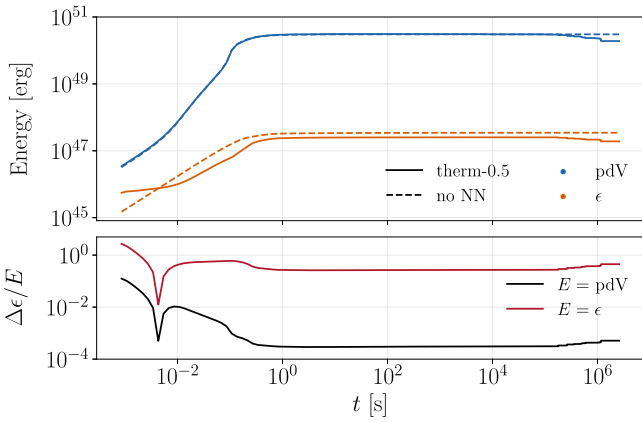
Figure 6. Top panel: evolution of total pressure work pdV (blue) and nuclear heating \epsilon = \dot{\epsilon}_{\text{nuc}} dt (orange) averaged all over the ejecta and integrated over time from the SNEC runs with (solid lines) and without (dashed lines) a coupled NN and a constant thermalization factor f_{\text{th}} = 0.5 . Bottom panel: difference in the nuclear heating between the two simulations normalized over pdV (black line) or \epsilon (red line) from the simulation using the heating rate fits.
