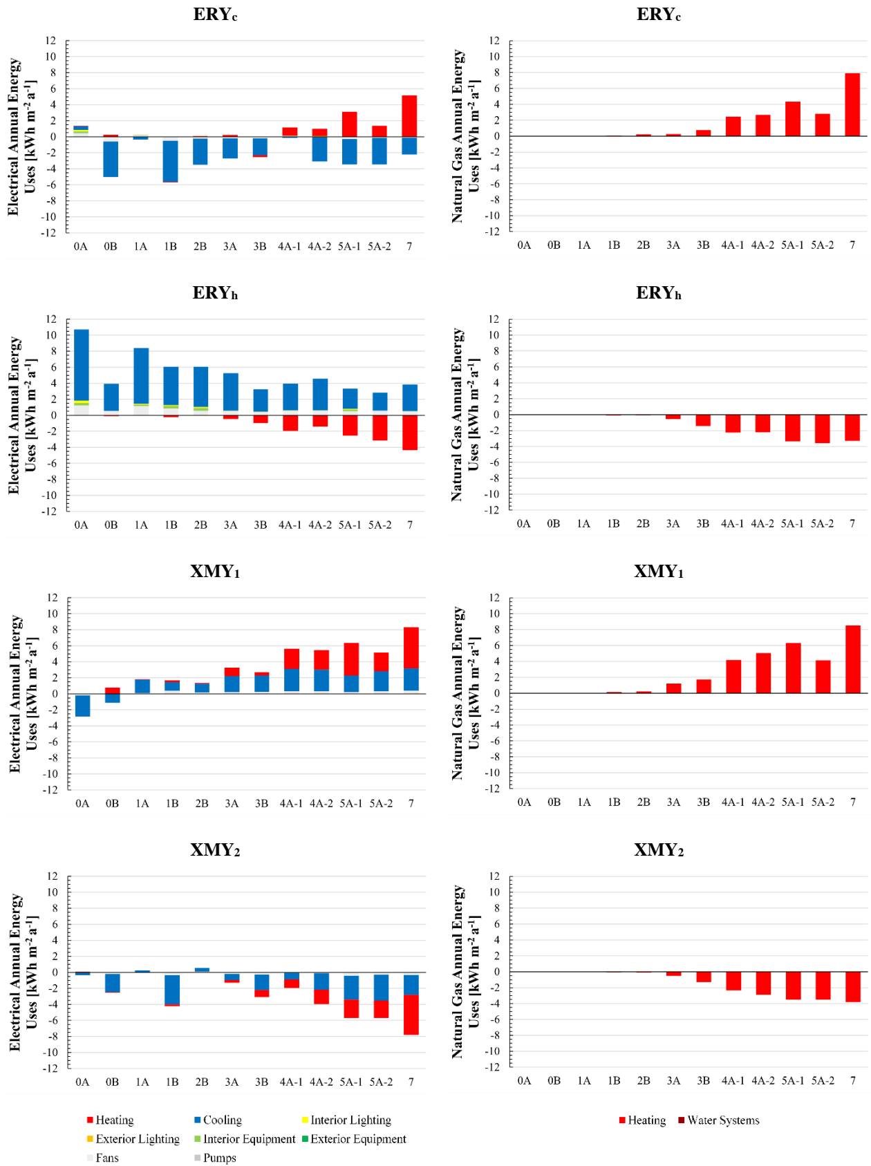
Figure 4: Deviation of final energy uses simulated with extreme years with respect to TMY x simulations: annual electrical energy uses (on the left) and annual natural gas uses (on the right).
