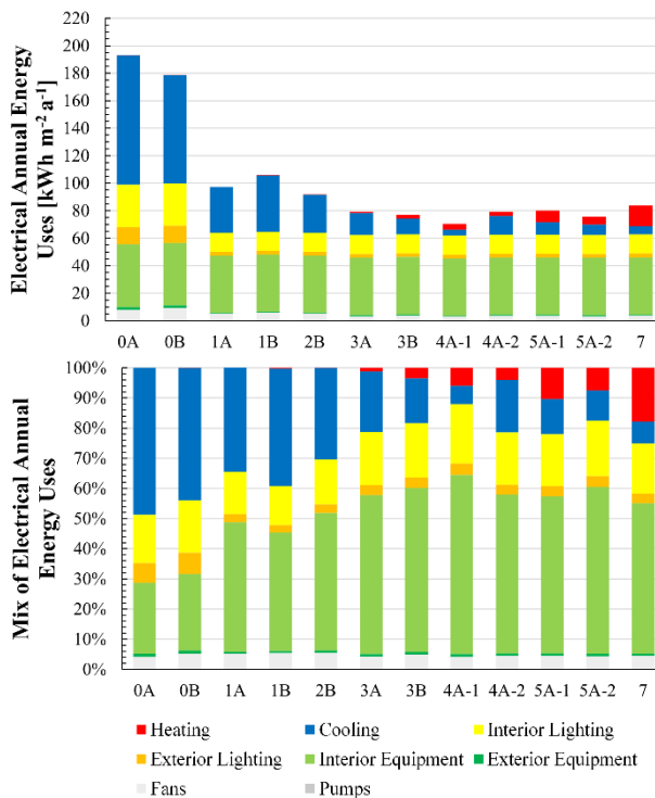
Figure 3: Results of TMY_x simulations: annual electrical energy uses (on the top left) and mixes (on the bottom left), and annual natural gas uses (on the top right) and mixes (on the bottom right).
