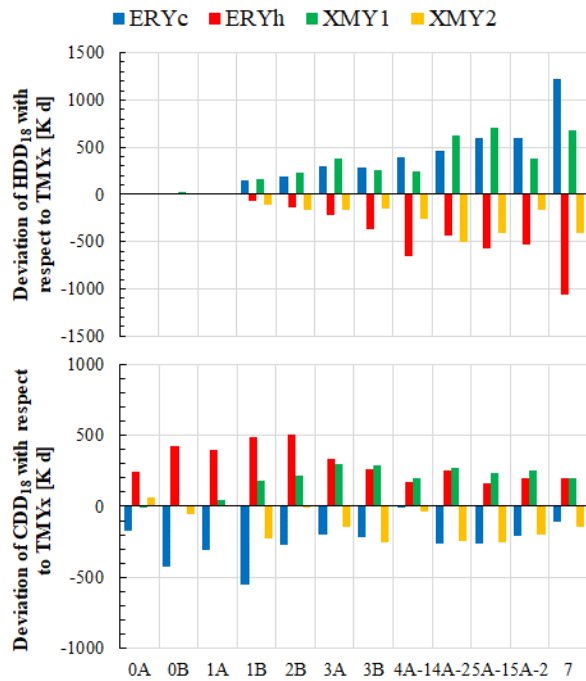
Figure 2: Deviation of HDD_{18} (top) and CDD_{18} (bottom) of ERY_c , ERY_h , XMY_1 and XMY_2 with respect to TMY_x .
