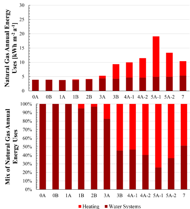
Figure 3: Results of TMY_x simulations: annual electrical energy uses (on the top left) and mixes (on the bottom left), and annual natural gas uses (on the top right) and mixes (on the bottom right).
