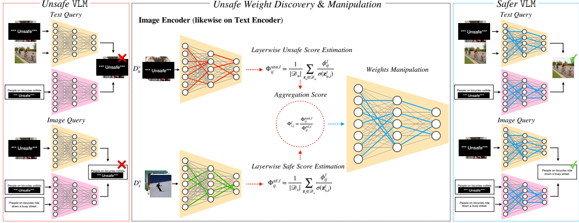
Figure 3. Unsafe Weights Manipulation (UWM) discovers unsafe weights of a given VLM and manipulates them to improve safety. Using safe and unsafe data within a single modality (e.g., the image modality shown in the center), UWM analyzes each encoder’s activations to estimate layer-wise safe and unsafe scores, which are then aggregated. Lastly, a small percentage of the top-scoring weights is targeted and manipulated towards safety. Applied independently to each encoder, UWM prevents cross-modal interference during scoring.
