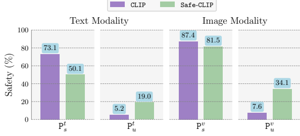
Figure 2. CLIP vs Safe-CLIP. The preference metrics P_s^t and P_u^t expose the degraded Safe-CLIP’s safety on safe queries.
