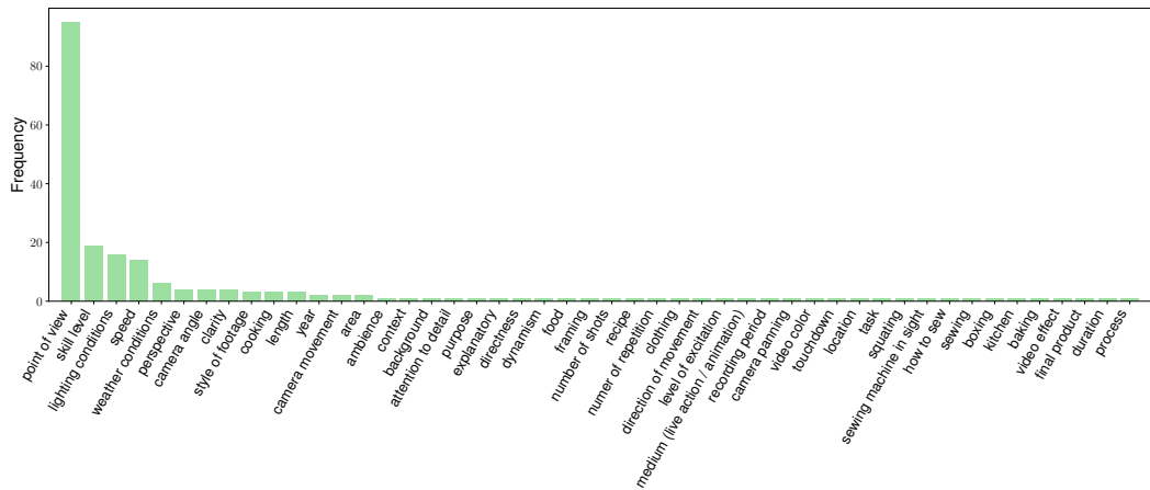
Figure 9: User-defined concepts.
