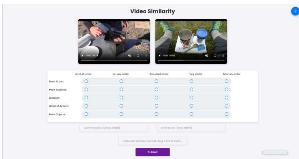
Figure 7: Annotation interface.
