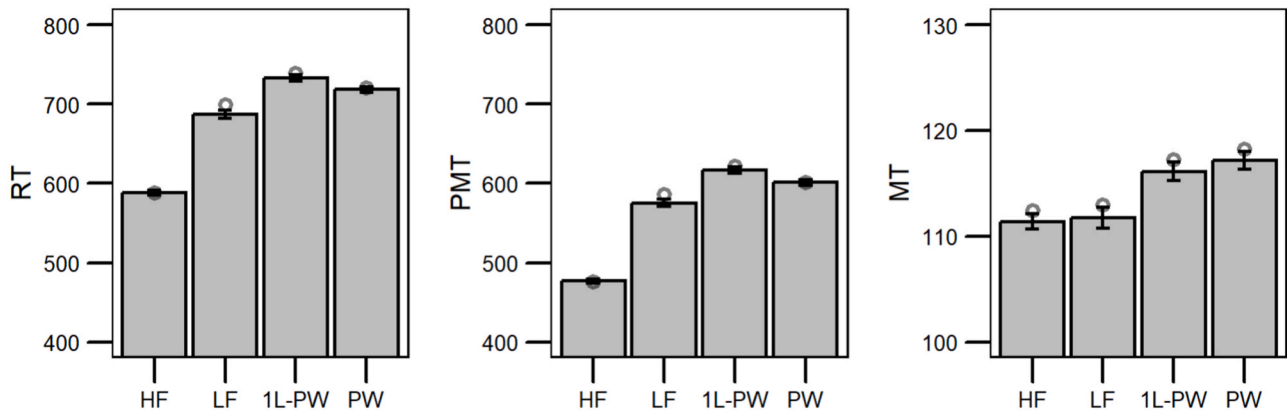
Fig. 1. Results for reaction time (RT), premotor time (PMT), and motor time (MT). Empty circles represent estimated marginal means. Error bars display 95% confidence intervals, adjusted for within-participants variables following Morey (2008). HF = high-frequency words; LF = low-frequency words; 1L-PW = one-letter pseudowords; PW = pseudowords.
