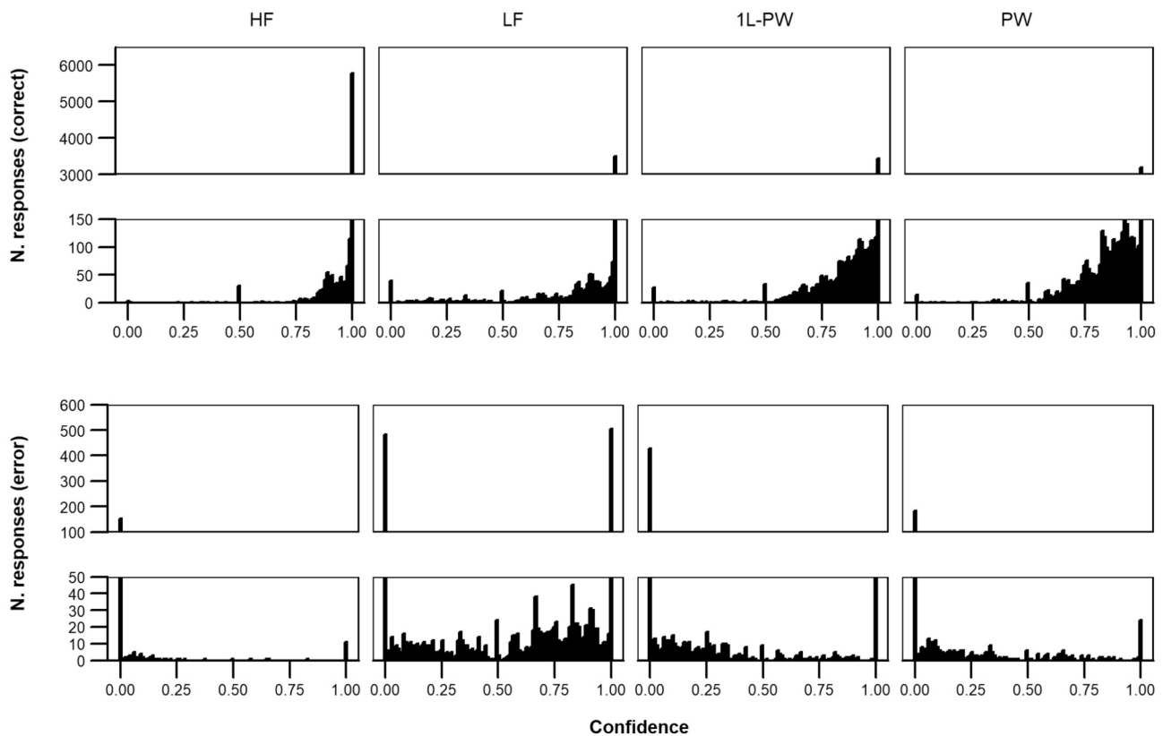
Fig. 3. Distribution of confidence ratings for correct and error responses as a function of stimulus types. HF = high-frequency words; LF = low-frequency words; 1L-PW = one-letter pseudowords; PW = pseudowords.
