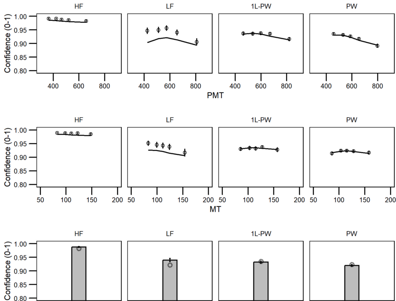
Fig. 4. Results of analyses of response confidence for correct responses. First and second row: points represent empirical scores and lines the estimated effect. Third row, empty circles represent estimated marginal means. Across figures, error bars display 95 % confidence intervals, adjusted for within-participants variables following Morey (2008). HF = high-frequency words; LF = low-frequency words; 1L-PW = one-letter pseudowords; PW = pseudowords.
