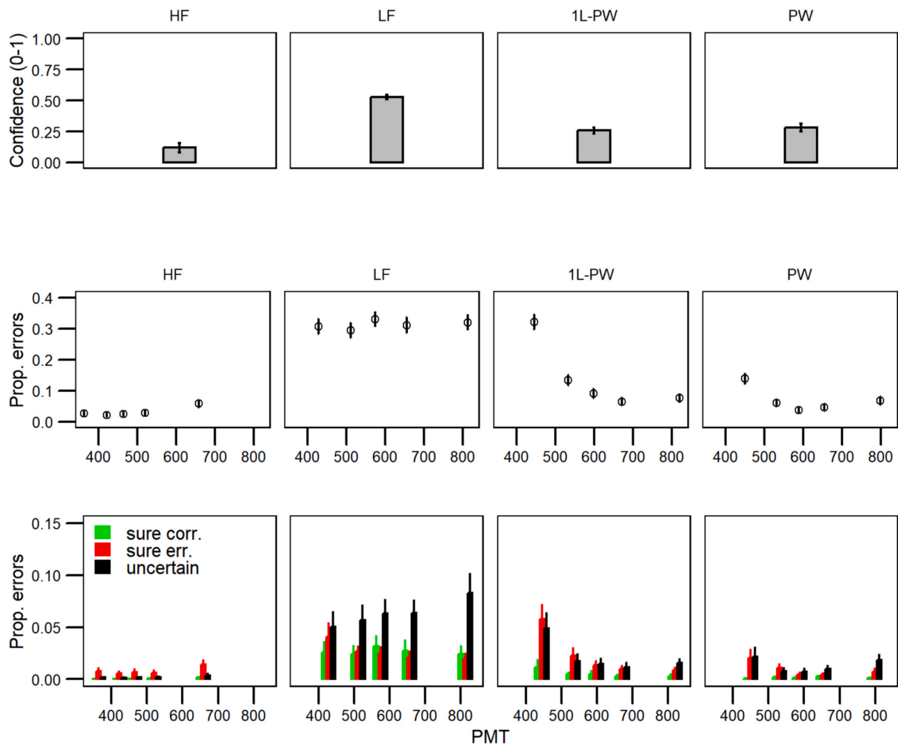
Fig. 5. Descriptive summary of response confidence for error responses. First row: overall average confidence as a function of stimulus type. Second row: Proportion of errors as a function of stimulus type and PMT quantile. Third row: data of the second row are broken down for different types of error (sure corr. = errors rated as correct responses with maximal confidence levels; sure err. = errors identified with maximal confidence; uncertain = errors rated between 0.01 and 0.99).
