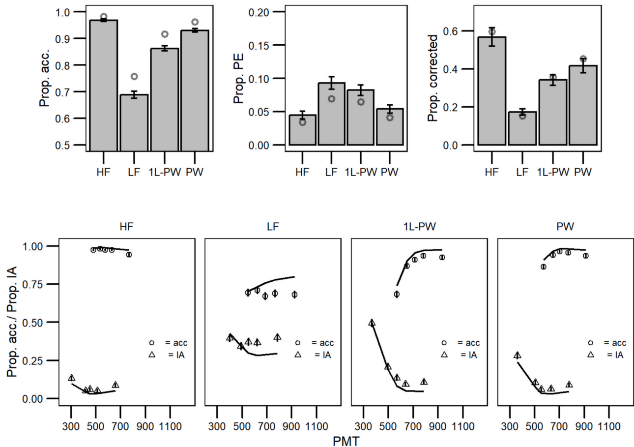
Fig. 2. Results for accuracy measures. First row: Results for accuracy (Prop. acc. = proportion of accurate responses), partial errors (Prop. PE = proportion of partial errors), and correction likelihood (Prop. corrected). Empty circles represent estimated marginal means. Second row: Conditional accuracy functions (Prop. acc.; circles) and conditional inaccurate activations functions (Prop. IA = proportion of incorrect activations; triangles) for each stimulus category. Error bars display 95 % confidence intervals, adjusted for within-participants variables following Morey (2008). Lines represent estimated marginal means. HF = high-frequency words; LF = low-frequency words; 1L-PW = one-letter pseudowords; PW = pseudowords.
