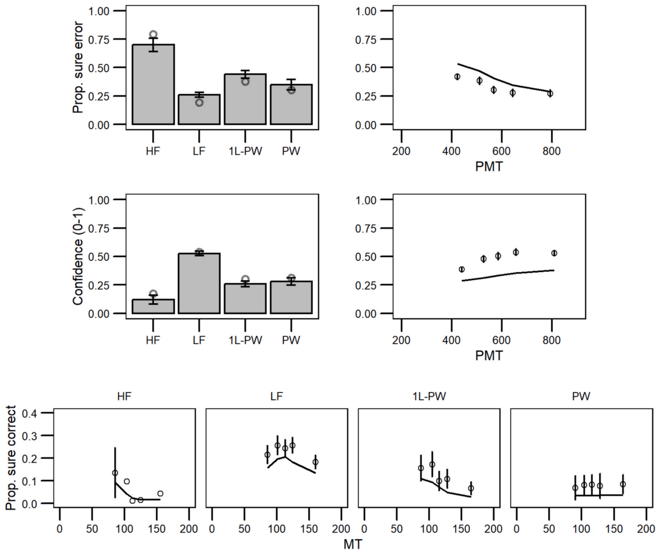
Fig. 6. Results of analyses of response confidence for error responses. First row: Effects of Stimulus Type and PMT Quantile on the likelihood of identifying errors with maximal confidence ( = 0 ). Second row: Effects of Stimulus Type and PMT Quantile on confidence ratings for uncertain errors (confidence = .01-.99 ). Third row: Stimulus Type by MT Quantile for the likelihood of rating errors as correct responses with maximal confidence ( = 1 ). Within bar plots, empty circles represent estimated marginal means. Within scatterplots, points represent empirical scores and lines the estimated effect. Error bars display 95 % confidence intervals, adjusted for within-participants variables following Morey (2008). HF = high-frequency words; LF = low-frequency words; 1L-PW = one-letter pseudowords; PW = pseudowords.
