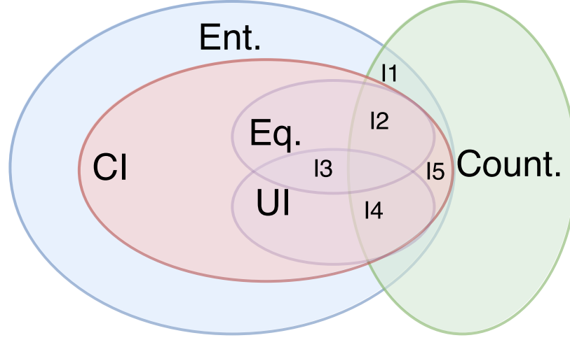
Figure 2.1: Constraint classes
