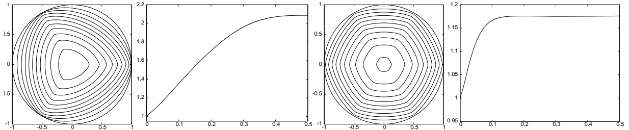
Figure 3: Anisotropic curvature flow for (6.7), with (k, \delta) = (3, 0.124) (left) and (6, 0.028) (right), using the scheme (5.4). Solution at times t = 0, 0.05, \dots, 0.5 . We also show plots of the ratio (6.2) over time.
