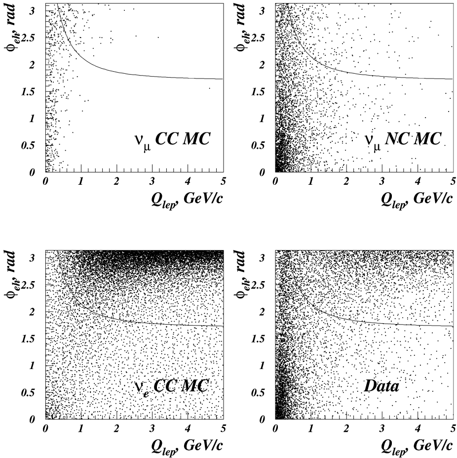
Fig. 2. The two-dimensional distributions \phi_{eh}-Q_{lep} (defined in the text) for Monte Carlo \nu_{\mu} CC and \nu_{\mu} NC (background) events and for \nu_e CC (signal) events, as well as for the NOMAD data. The events to the right of the curve were selected.
