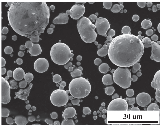
Fig. 1. SEM image of sterling silver powder.
