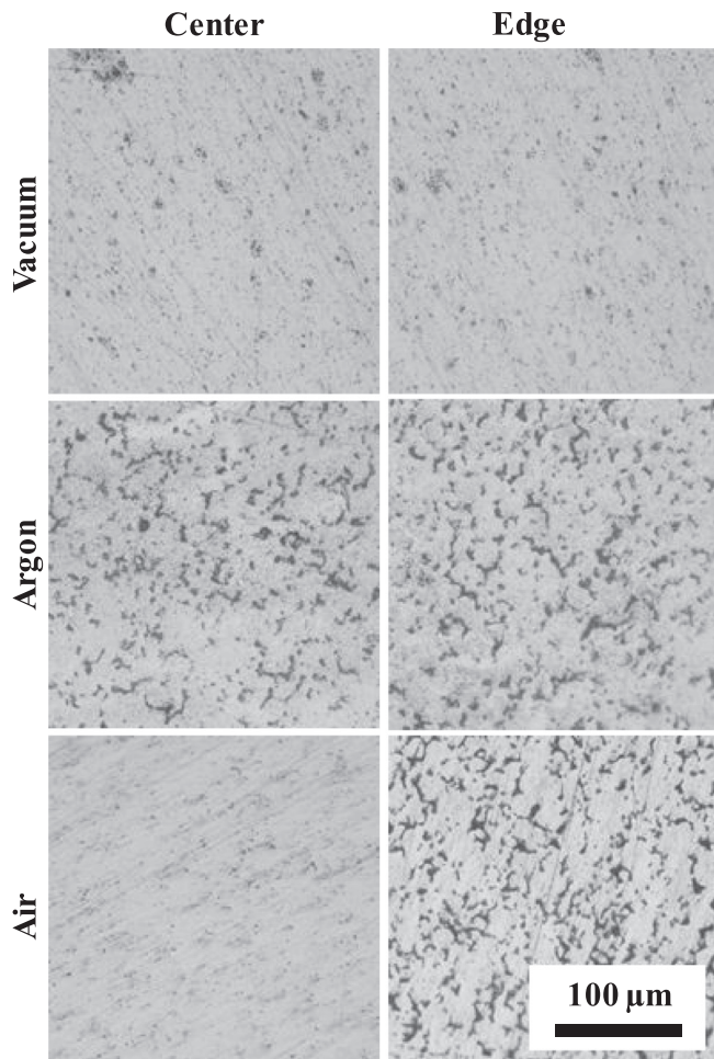
Fig. 4. Microstructures of the sintered silver samples in vacuum, argon and air in the center and the edge of the specimens (with black areas indicating the porosity), thermal cycle: 25 K/min to 550 °C, 2 K/min to 770 °C and 3 h of holding at 770 °C.
