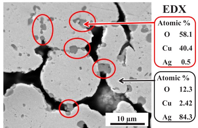
Fig. 5. Edge microstructure and EDX analysis of the air sintered silver sample.
