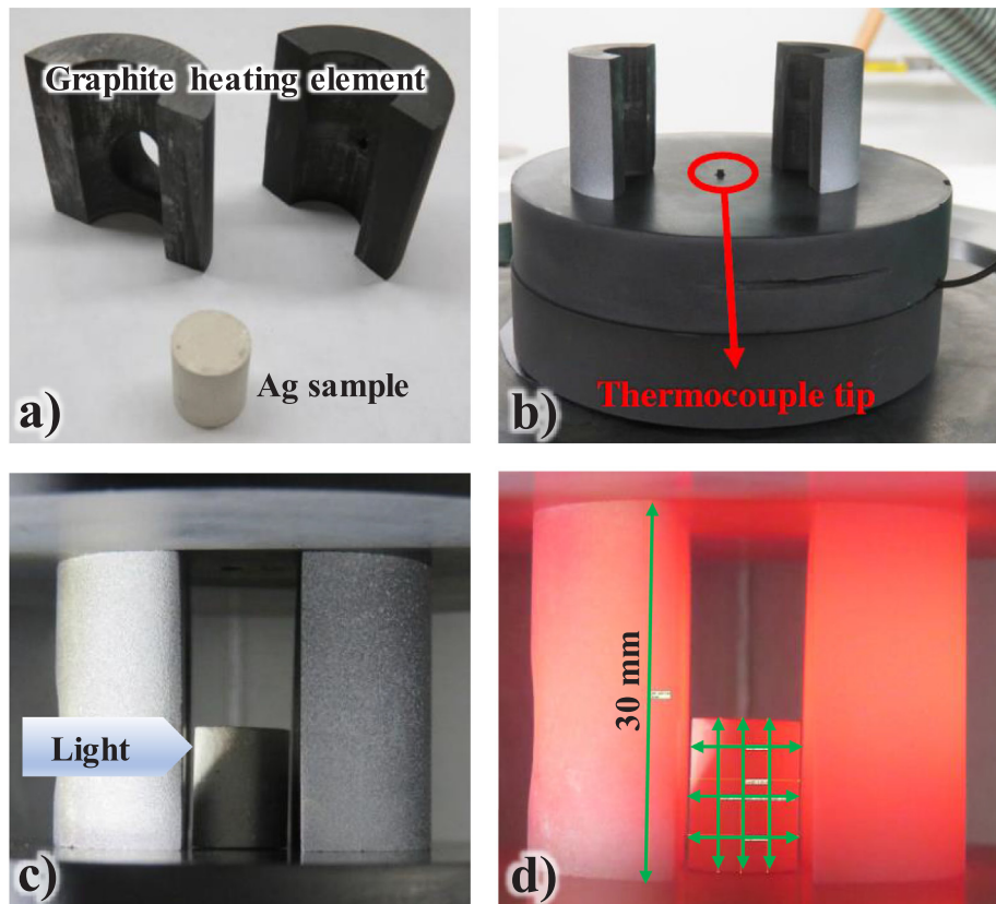
Fig. 2. Pressure-less vacuum SPS configuration with: (a) the Ag sample and graphite heating elements, (b) the thermocouple location, and the assembly at (c) low and (d) high temperature.
