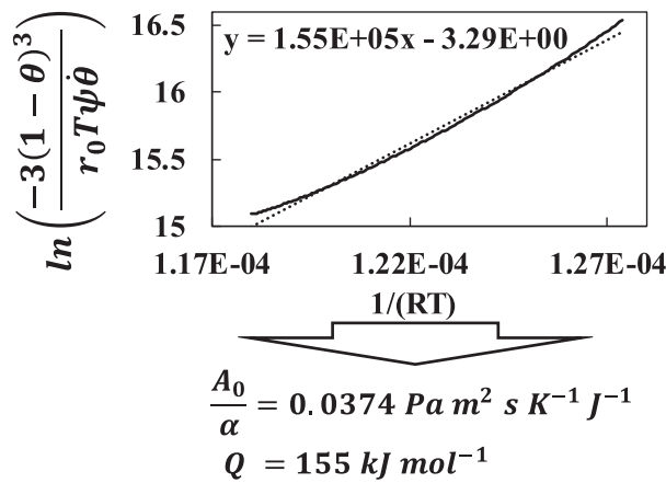
Fig. 6. Determination of the pressure-less sintering parameters by regression method (the dotted curve is the fitting curve).
