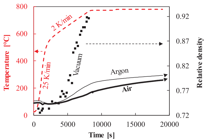
Fig. 3. Relative density curves (in black) of silver samples in vacuum, argon and air, the same thermal cycle is imposed onto the samples and is reported in red. (For interpretation of the references to color in this figure legend, the reader is referred to the web version of this article.)
