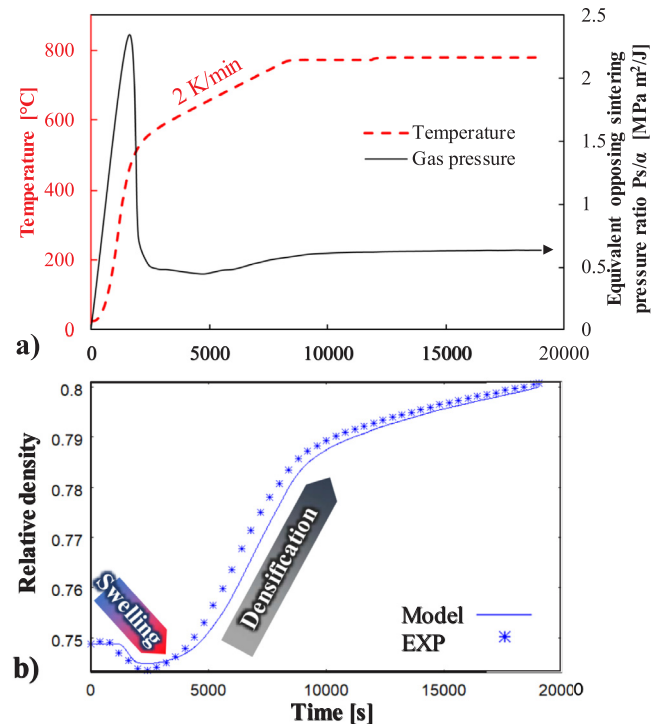
Fig. 8. (a) Sample temperature and equivalent opposing sintering pressure P_s/\alpha for the argon sintered sample, (b) modeling results for the sintering in argon test including the internal gas pressure term versus experimental data.
