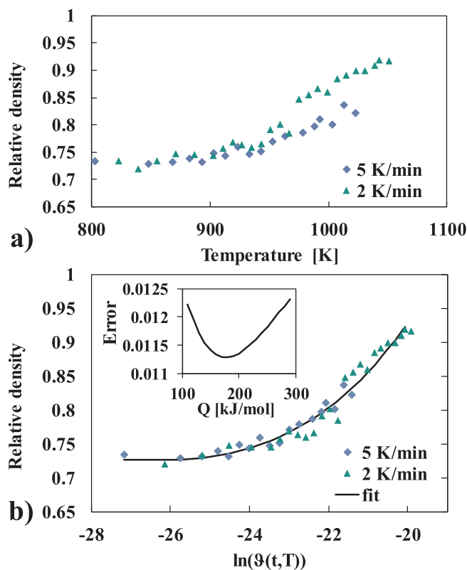
Fig. 7. Vacuum sintered densification curves at 2 and 5 K/min, (b) determination of the sintering activation energy by master sintering curve approach.
