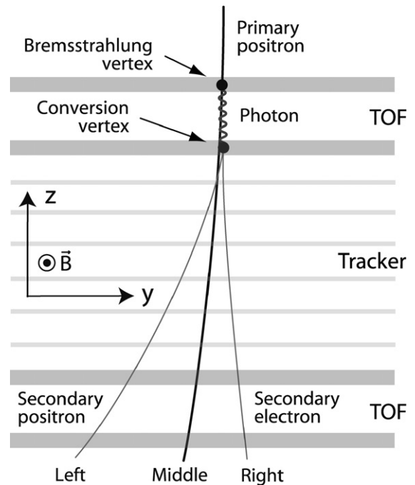
Fig. 1. Schematic view of a converted bremsstrahlung event caused by a positron going top-down.
