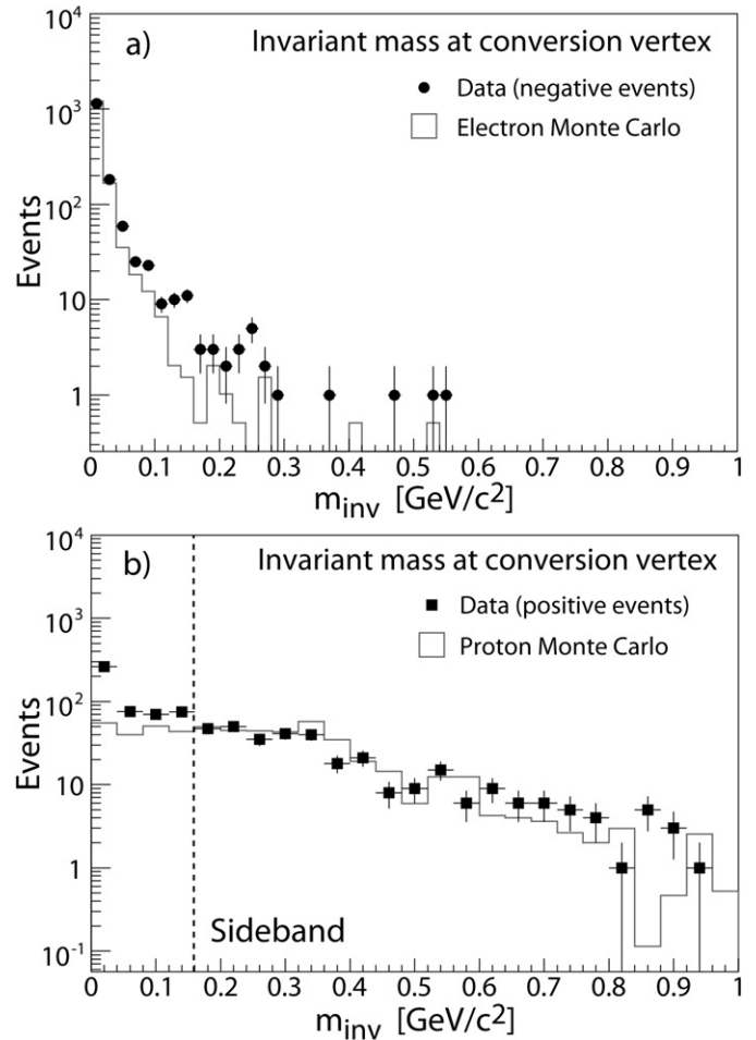
Fig. 2. (a) Invariant mass distribution at the conversion vertex for negatively charged data events (circles) and electron Monte Carlo (histogram). (b) The same display for positively charged data events (squares) and proton Monte Carlo (histogram). The proton Monte Carlo distribution has been scaled to the data using the sideband. Below the sideband threshold of 0.16 \text{ GeV}/c^2 , the excess in the data due to the positron contribution is apparent.
