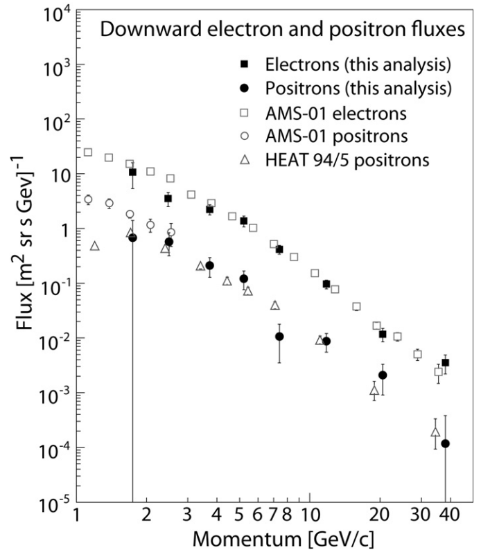
Fig. 7. The fluxes of downward going positrons (filled circles) and electrons (filled squares) measured in this analysis, compared with earlier results from AMS-01 (open circles and squares) [12] and HEAT- e^\pm (triangles) [4]. Error bars denote statistical errors only.
