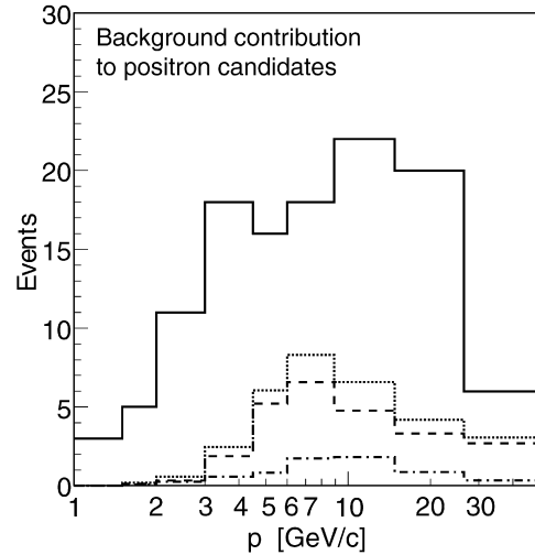
Fig. 3. Momentum distribution of the positron candidates including background (solid line) and the total estimated background (dotted line), itemized into contributions from protons (dashed line) and wrongly identified electrons (dash-dotted line).
