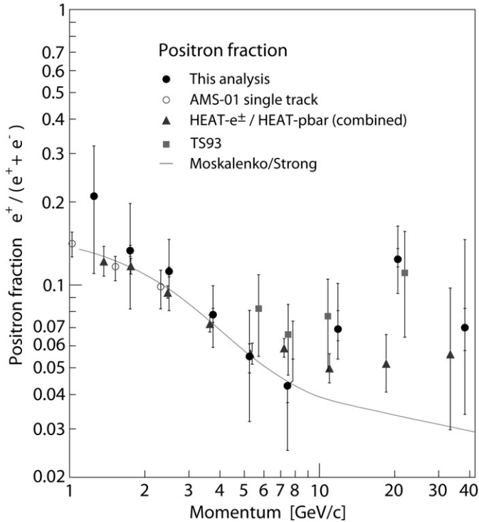
Fig. 4. The positron fraction e^+/(e^+ + e^-) measured in this analysis (filled circles), compared with earlier results from AMS-01 (open circles) [12], TS93 (squares) [13], the combined results from HEAT- e^\pm and HEAT-pbar (triangles) [14], together with a model calculation for purely secondary positron production from [15] (solid line). The total error is given by the outer error bars, while the inner bars represent the systematic contribution to the total error.
