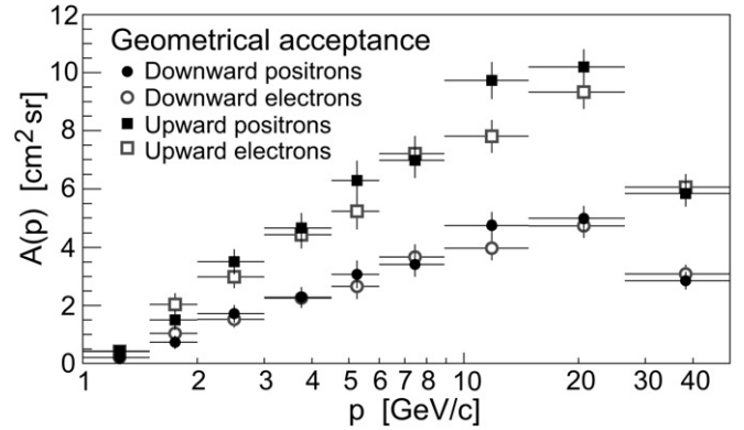
Fig. 5. The geometrical acceptance for downward (circles) and upward (squares) going positrons (filled) and electrons (open), when identified through bremsstrahlung conversion.
