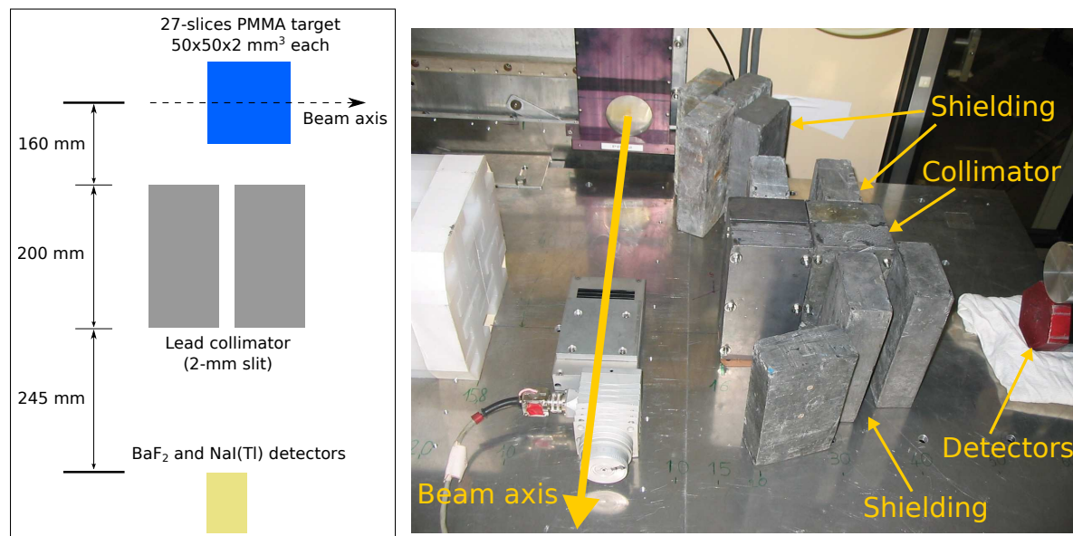
Figure 1: A schematic illustration (left) and a picture (right) of the GANIL 95 MeV/u ^{12}\text{C}^{6+} experiments. It should be noted that the target is not shown in the picture and that the schematic illustration is not to scale.
