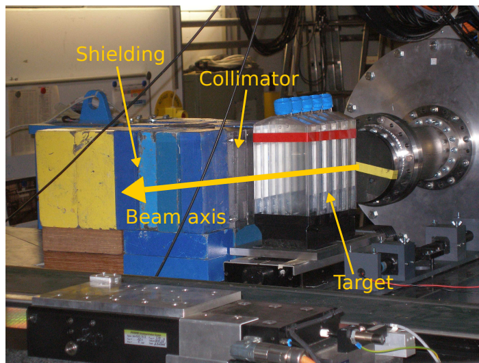
Figure 3: A schematic illustration (left) and a picture (right) of the GSI 310 MeV/u ^{12}\text{C}^{6+} experiment. It should be noted that the detector is not visible in the picture and that the schematic illustration is not to scale.
