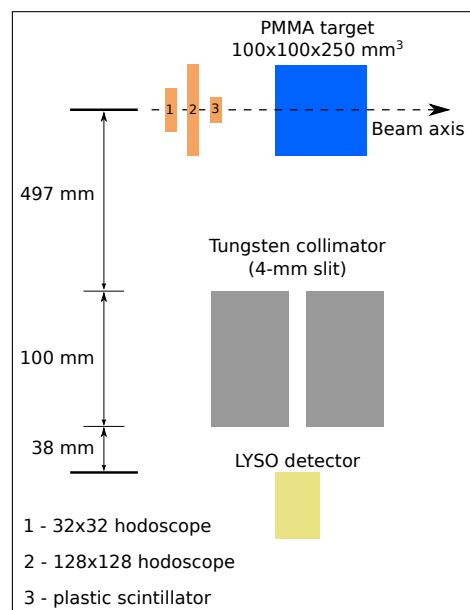
Figure 4: A schematic illustration (left) and a picture (right) of the HIT 310 MeV/u ^{12}\text{C}^{6+} experiment. The schematic illustration is not to scale.
