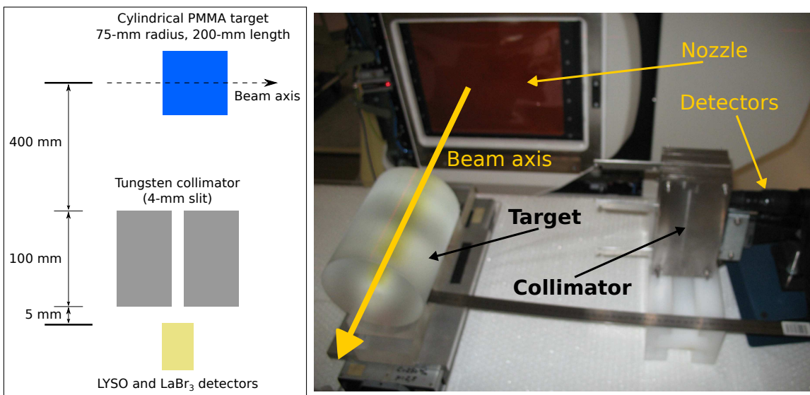
Figure 6: A schematic illustration (left) and a picture (right) of the WPE 160 MeV (II) proton experiments. The schematic illustration is not to scale.
