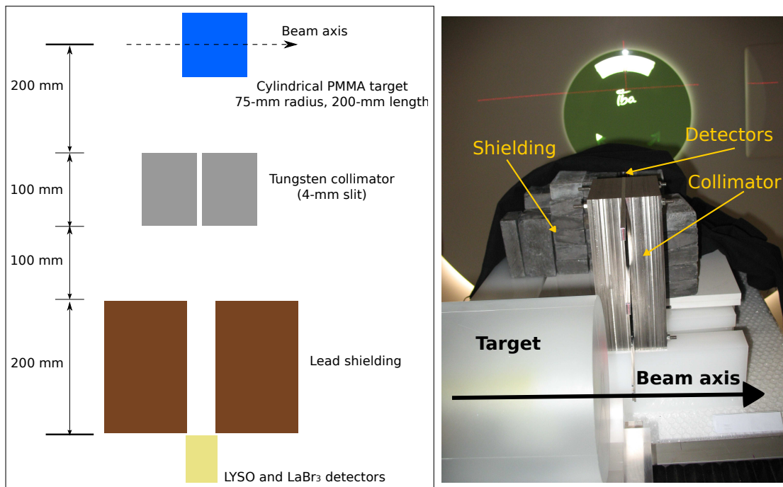
Figure 5: A schematic illustration (left) and a picture (right) of the WPE 160 MeV (I) protons experiments. The schematic illustration is not to scale.
