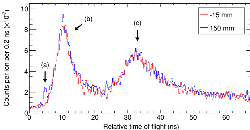
Figure 7: TOF spectra of the GSI 310 MeV/u ^{12}\text{C}^{6+} experiment for the measurement points at -15 mm (upstream of the target) and 150 mm (inside the target). The TOF components corresponding to the events associated with prompt gammas (a), secondary-induced events from the target ((b), mainly neutron-associated events), and events associated with the surroundings ((c), e.g. walls, ceiling) are pointed out by arrows and have been suggested by Testa et al (2010). The X-axis is relative since no calibration for the axis origin was performed.
