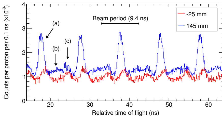
Figure 8: Comparison between two TOF spectra obtained for two longitudinal positions (25 mm upstream of the target and 145 mm inside the target). These data come from the WPE 160 MeV H + (II) experiment using the LaBr 3 detector and they include five proton bunches (9.4-ns beam period). The prompt-gamma events (a), the secondary-induced events (b), and the events originated in the nozzle (c) are pointed out by arrows. The nozzle-related events in these data have been already discussed by Pinto et al (2014). The X-axis is relative since no calibration for the axis origin was performed.
