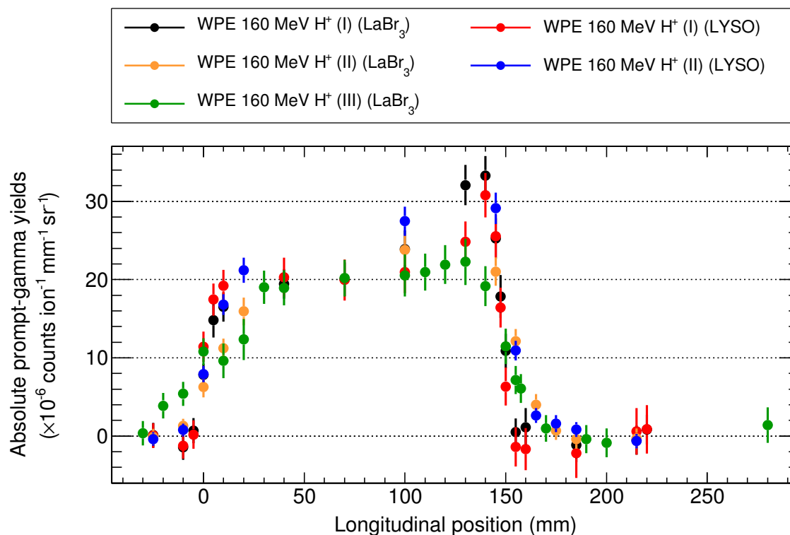
Figure 15: Profiles of the proton experiments after full normalization. Each data point includes both statistical (one standard deviation) and the considered systematic uncertainties.
