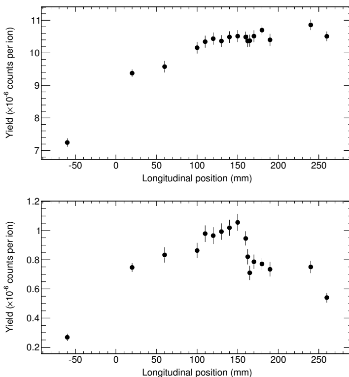
Figure 11: Profiles of the HIT 310 MeV/u ^{12}\text{C}^{6+} experiment, LYSO detector, without using TOF (top) and using TOF (bottom). The error bars correspond only to statistical uncertainties (one standard deviation).
