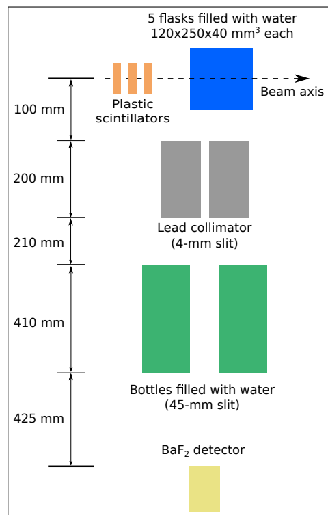
Figure 3: A schematic illustration (left) and a picture (right) of the GSI 310 MeV/u ^{12}\text{C}^{6+} experiment. It should be noted that the detector is not visible in the picture and that the schematic illustration is not to scale.
