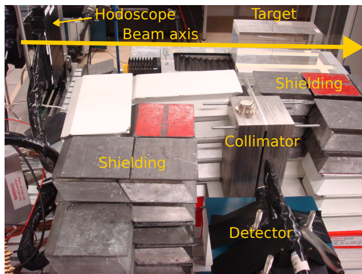
Figure 4: A schematic illustration (left) and a picture (right) of the HIT 310 MeV/u ^{12}\text{C}^{6+} experiment. The schematic illustration is not to scale.
