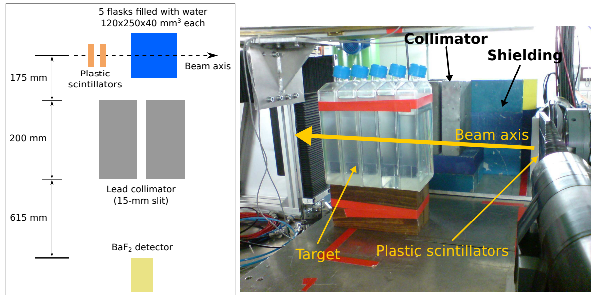
Figure 2: A schematic illustration (left) and a picture (right) of the GSI 300 MeV/u ^{12}\text{C}^{6+} experiment. It should be noted that the detector is not visible in the picture and that the schematic illustration is not to scale.
