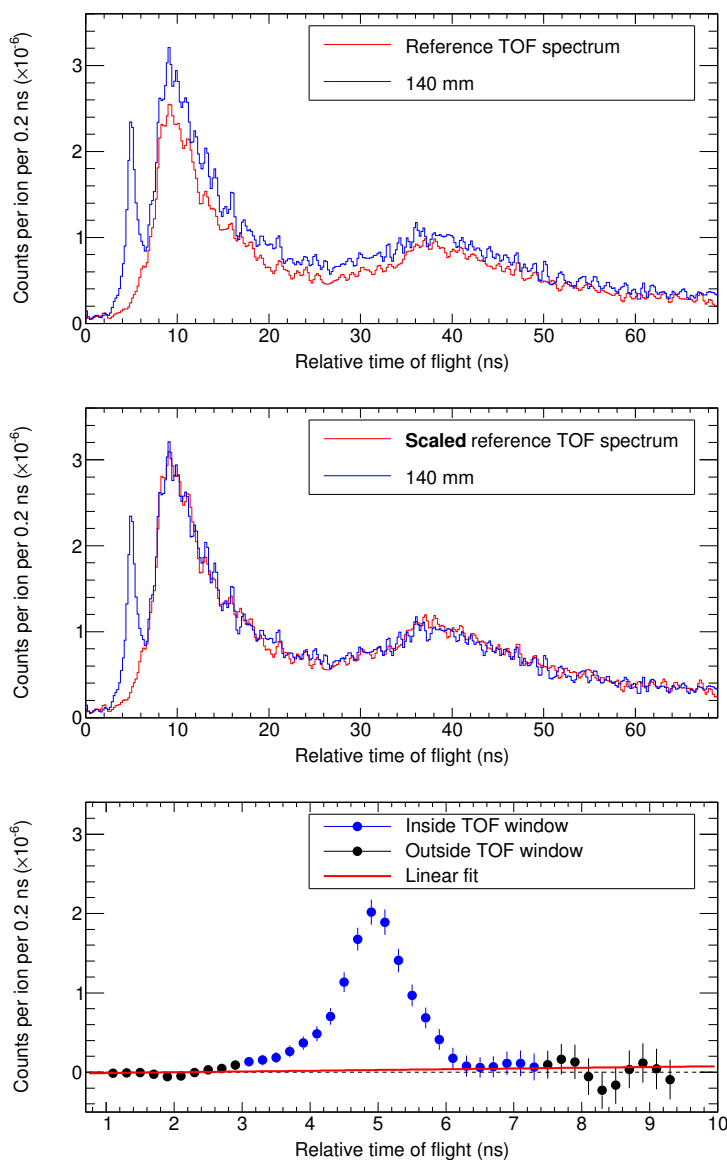
Figure 12: Different steps of the background subtraction procedure using the GSI 300 MeV/u ^{12}\text{C}^{6+} experiment and the measurement at 140 mm inside the target as an example. Top: TOF spectrum to be subtracted and the reference one. Middle: reference TOF spectrum scaled in order to account for the difference in background magnitude. Bottom: TOF region around the prompt-gamma peak after background subtraction.
