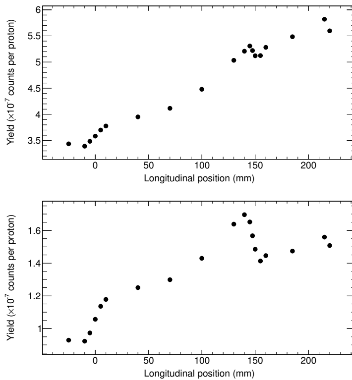
Figure 10: Profiles of the WPE 160 MeV H^+ (I) experiment, LaBr_3 detector, without using TOF (top) and using TOF (bottom). The error bars are of the same size as the symbols and correspond only to statistical uncertainties (one standard deviation).
