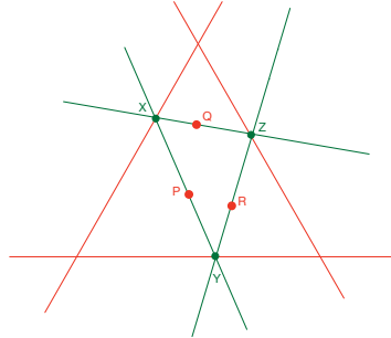
FIGURE 1. Description of \mathfrak{T}(P, Q, R) : the fixed data are red, the variable data are green
