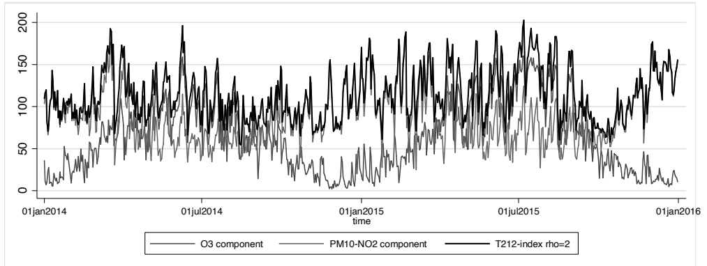
Figure 5. The two pollutant components and the T2-aggregate AQI for \rho=2
