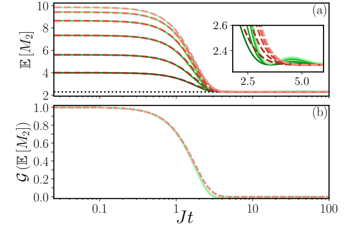
FIG. 6. Comparison of ED and ME results for M_2 of \hat{R} , with N = 8 . Colors and shading of ED (solid) and ME (dashed) curves are as in Fig. 2. The analytically predicted steady-state value of Eq. (22) for the half-filling sector is given by the black dotted line. (a) For each initial state, the ME simulation reproduces the exact dynamics very well. There is a discrepancy at intermediate times due to non-Markovian effects not captured by the ME (inset). (b) The ME reproduces the collapse to a universal curve under rescaling (4).
