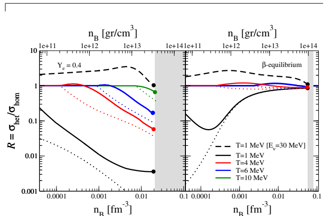
FIG. 6. Ratio \mathcal{R} from Eq.(13) in two different conditions: fixed proton fraction Y_e = 0.4 (left panel) and \beta -equilibrium (right panel). The gray band indicates the region in density where non-spherical pasta may be present, and the curves terminate with a dot for the density at which u = 1/8 . Dotted curves indicate the contribution of the external gas only. Neutrinos are considered at thermal equilibrium, except for the black dashed curves where E_\nu = 30 MeV.
