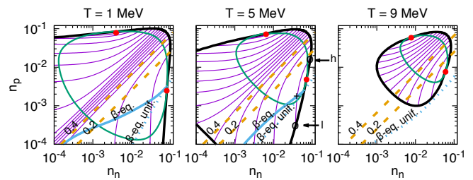
FIG. 1. \beta -equilibrium path (blue line) for SLy4 Skyrme interaction in the coexistence region (delimited by the solid black symbols) in the (n_n, n_p) plane and for T=1-9 \text{ MeV} . A sample of the Gibbs construction paths are shown (purple lines). The global density which intersect the \beta -equilibrium path in blue solid line with the Gibbs construction one (see for instance the "+" symbol at T=5 \text{ MeV} ), represents the equilibrium state connecting the 2 phases at equilibrium which are located at the boundaries (see the points labelled l and h which are the low and high density phases associated to the global density identified by the "+" symbol at \beta -equilibrium). The constant Y_e = 0.2, 0.3 and 0.4 paths are represented by the yellow dashed lines. The spinodal instability region is also shown (green line) and the critical points are shown with red solid dots with error-bars.
