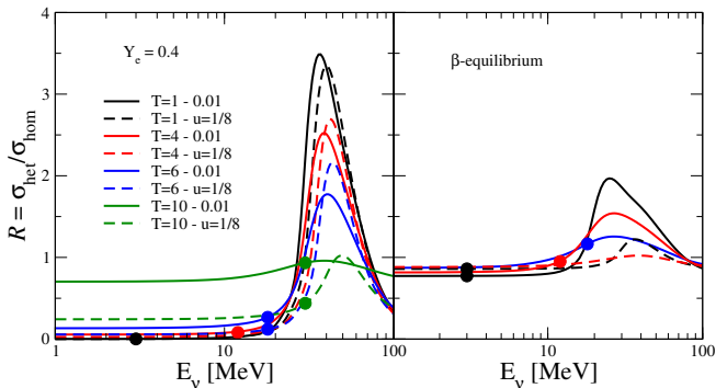
FIG. 7. Energy dependence of the total ratio of cross section \mathcal{R} at various temperatures and for two different densities: n_B = 0.01 \text{ fm}^{-3} (full lines) and the threshold density for which u = 1/8 (dashed lines). As for Fig.6 the left panel is for fixed proton fraction Y_e = 0.4 and the right panel is for \beta -equilibrium conditions. In both cases the full dots indicate the energy for thermal neutrinos ( E_\nu = 3T ).
