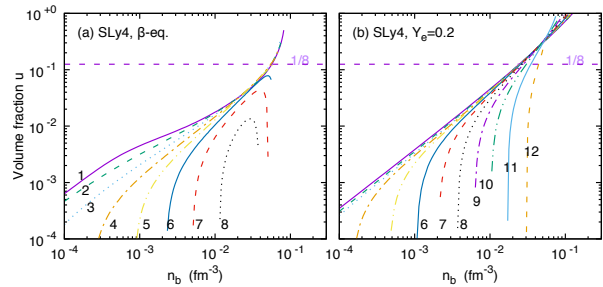
FIG. 2. Volume fraction of the high density phase in heterogeneous matter for SLy4 Skyrme interaction. (a) for the \beta -equilibrium path, (b) for the constant Y_e = 0.2 path.
