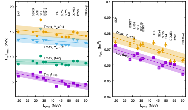
FIG. 5. (a) Melting temperature T_m and maximal temperatures T_{max} at \beta -equilibrium, compared to T_{max} at fixed x_e=0.2 and 0.4 for the set of EOS compatible with chiral EFT EOS in neutron matter. (b) Highest density reached by the pasta phase for beta equilibrium or at fixed Y_e . These predictions are shown versus L_{sym} .
