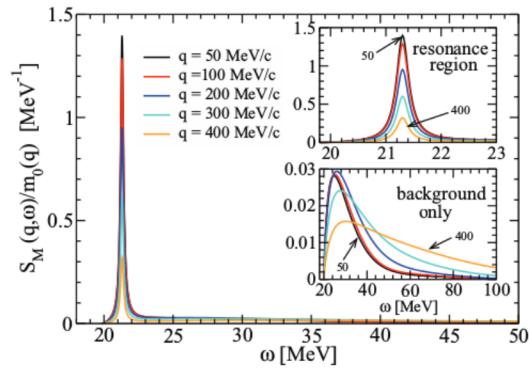
FIG. 2. (Color online) S_M(q, \omega)/m_0(q) for various fixed q . In the insets the strength in the resonance region and the background contribution [40].
