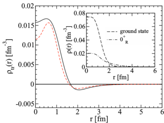
FIG. 1. (Color online) Transition density between the ground state and the 0_R^+ for the chiral (black full line) and the phenomenological (red [gray] dashed line) forces. In the inset the densities of the ground state and of the 0_R^+ for the chiral force are also shown.
