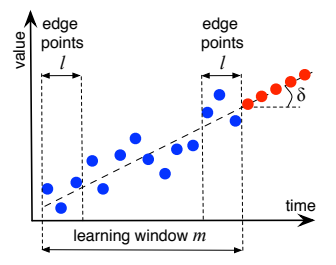
Fig. 2. Derivative-based Prediction.
