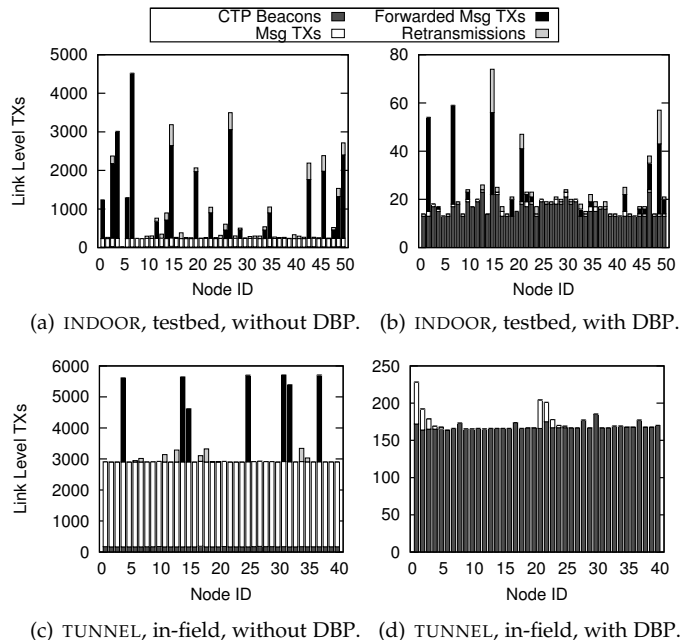
Fig. 14. Link-level transmissions with and without DBP for INDOOR, testbed (2 h) and TUNNEL, in-field (23 h). Note the varying y -axis scale.
