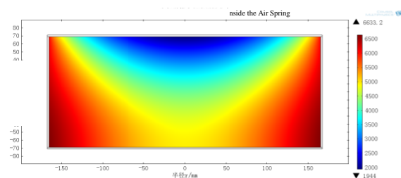
Figure 3. Sound pressure field distribution in cylindrical air spring with flexible shell.
