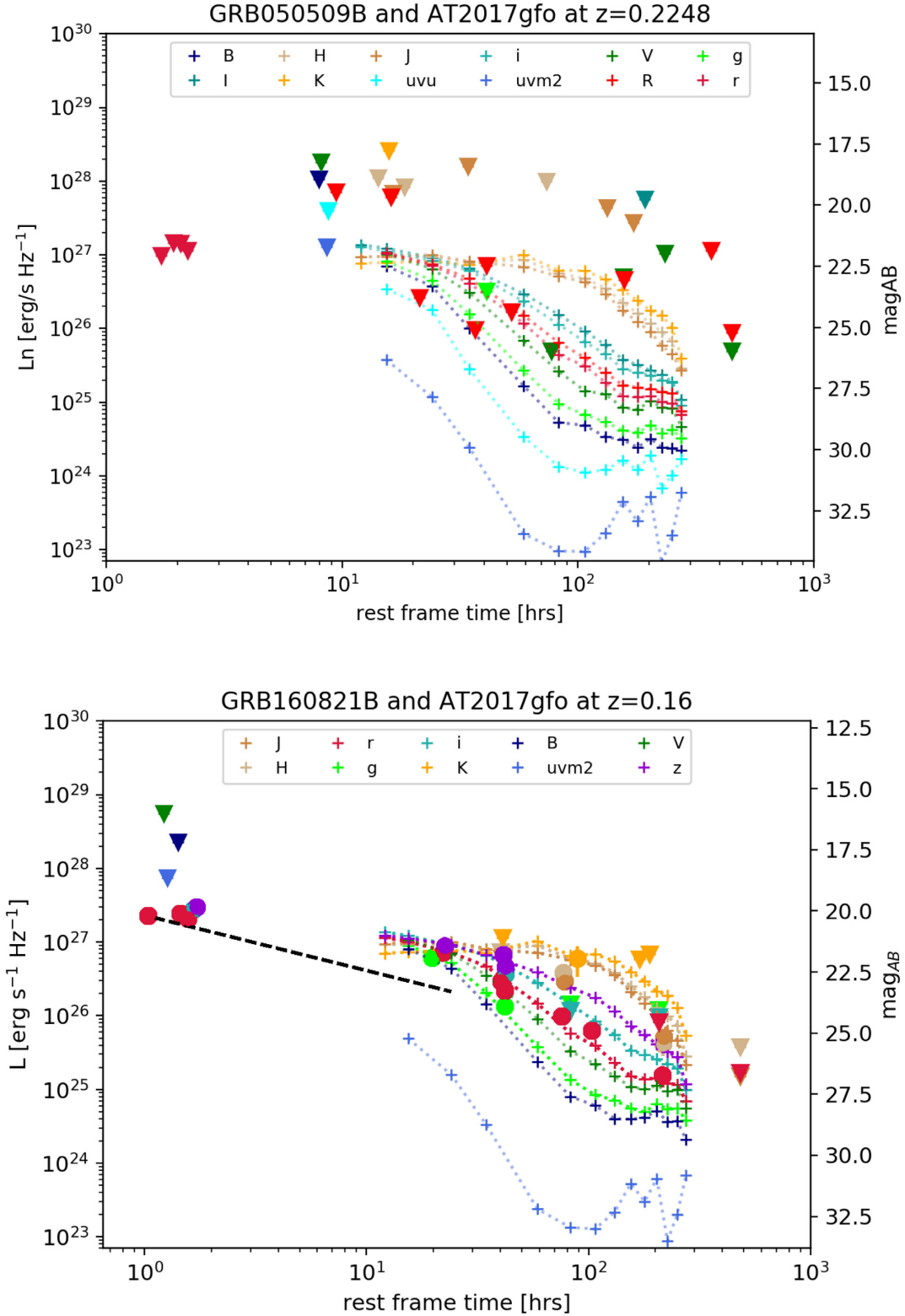
Figure 4. Two examples of short GRBs for which the optical counterpart luminosity (circle for a detection and triangle for an upper limit) is fainter than AT2017gfo luminosity (dotted lines with crosses) in at least one effective rest-frame filter (see Section 3.2 for effective rest-frame filter definition). See Fig. A1 for the full sample of short GRBs with similar properties. Note that GRB 160821B ( lower panel ) shows evidence of a temporal decay index lower than the shallowest index predicted by the fireball model (i.e. \alpha = 0.75 , see Section 4.2, black dashed line). If this anomalous shallow decay is due to an emerging KN emission, its NIR luminosity is a factor of 1.2–2 fainter than AT2017gfo at epochs later than 3 d after the merger time in r and J bands (see Table 2).
