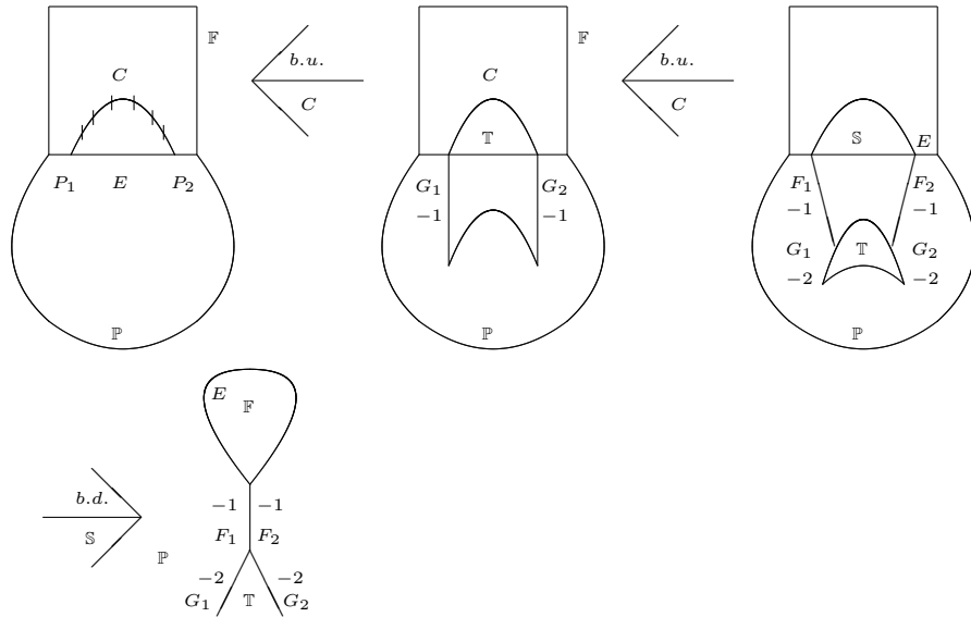
FIGURE 2. The 2-throw operation of the double curve C .
