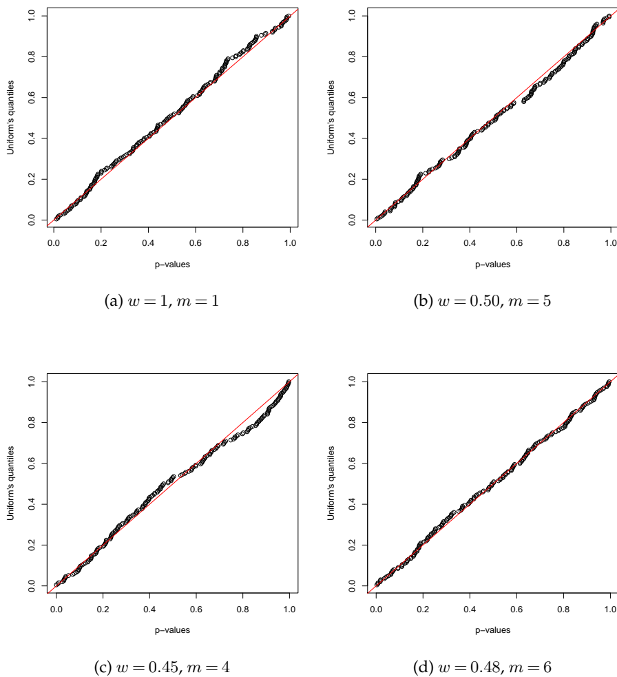
Figure 7: We present some qqplots of p-values versus the quantiles of a Uniform distribution, simulations performed using different parameter settings.
