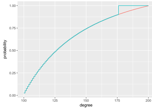
Figure 3: Under H_0 degree distribution is the red conditional de Solla Price power-law, whereas under H_1 the degree distribution is taken to be the blue step function with h_c = 0.1 and c = 100 .
