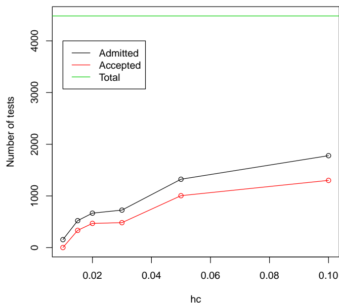
Figure 4: The green line shows the overall number of 4482 degree distributions that are possible to test. The black line shows the number of admissible tests that have power greater than 80% with respect of tail sensitivity h_c . The red line illustrates the number of test for which the de Solla Price power-law seems to be a sensible model.
