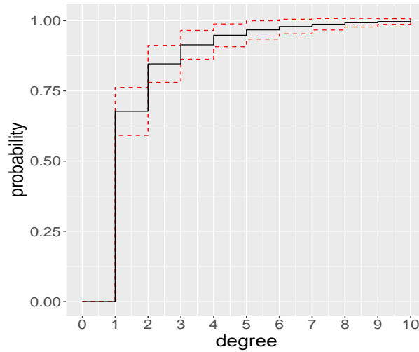
Figure 1: An example of a de Solla Price cumulative degree distribution; dashed lines indicate the standard deviation of the empirical degree distribution considering a network of size 30.
