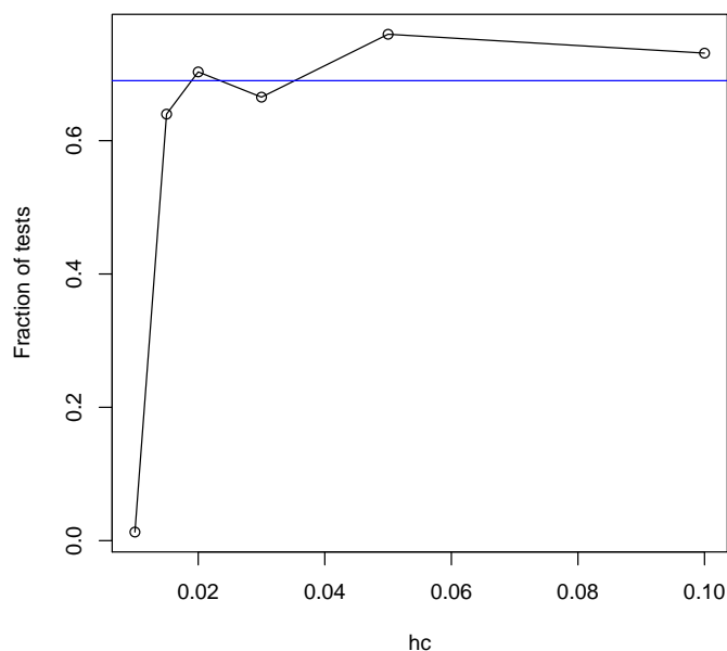
Figure 5: Fraction of accepted tests, i.e., rate of detected power-law networks, for h_c = [0.01, 0.015, 0.02, 0.03, 0.05, 0.1] . Note that the rate is stable for h_c > 0.01 . This suggests that roughly 2/3 of all considered real-world networks seem to exhibit power-law tail behaviour.
