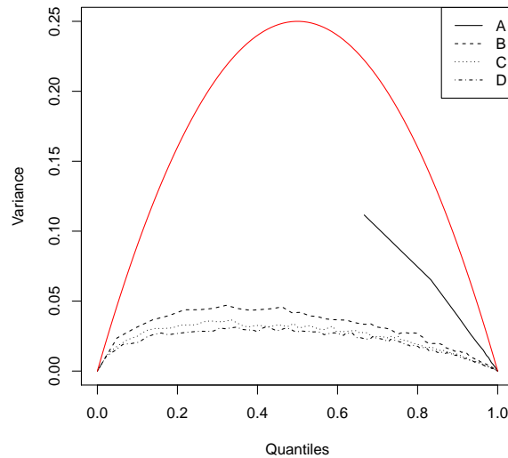
Figure 2: Brownian Bridge's empirical variance with A:( w=1 , m=1 ), B:( w=134 , m=23 ), C:( w=267 , m=44 ), D:( w=400 , m=51 ). Red line is the variance under independent degree sampling (see Appendix A). Line A is complete, but starts from the first rescaled degree F^{\text{SP}}(0; 1, 1) = 0.66 .
