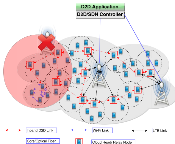
FIGURE 4. Extending coverage area in case of disaster and traffic hotspot situation.
