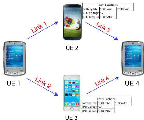
FIGURE 6. Example of route selection for different cost functions.
