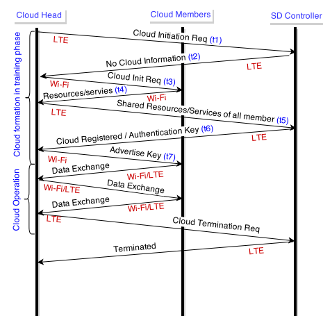
FIGURE 2. Description of signaling for cloud formation.
