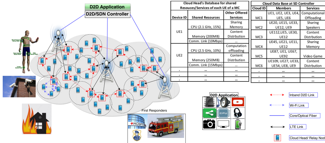
FIGURE 1. The proposed Software-Defined D2D communication architecture for public safety applications.
