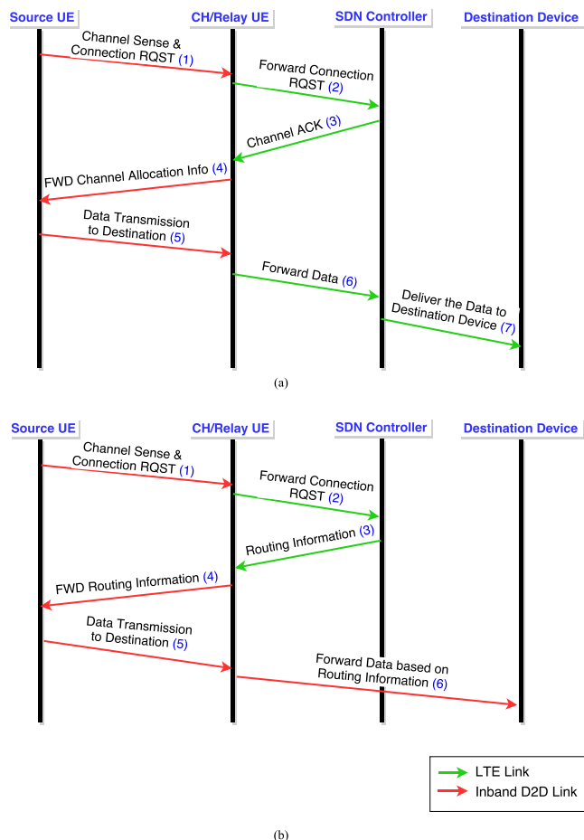
FIGURE 5. Signaling for multi-hop routing between cloud heads. (a) Adequate resource available in eNB. (b) The eNB is fully loaded, computes a route information.
