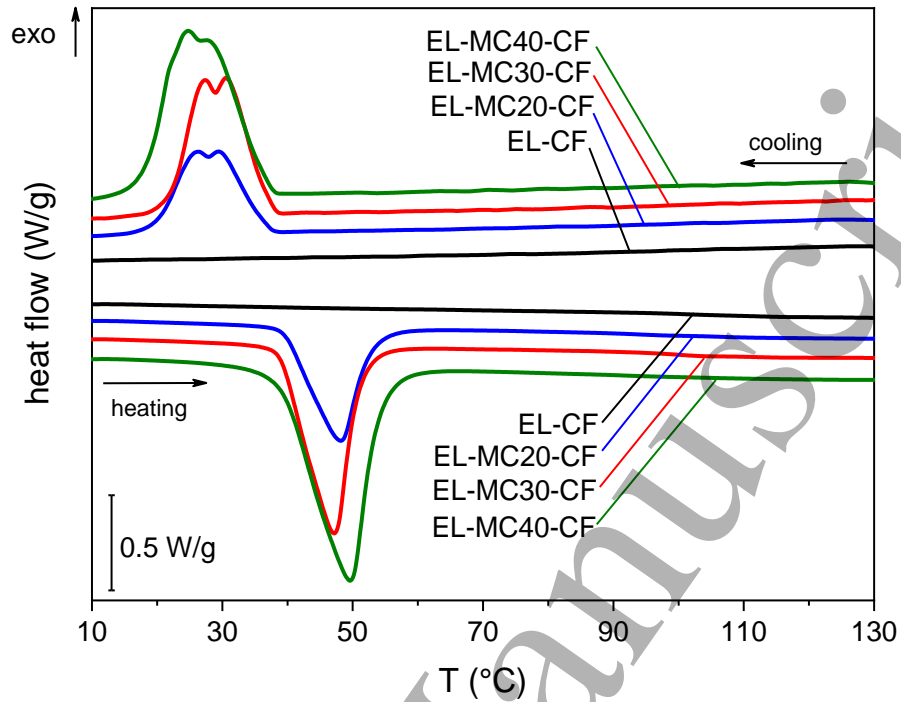
Figure 18. DSC thermograms of the samples EL-MC x -CF (10 °C/min; N 2 flow = 100 ml/min) (data from [158]).
