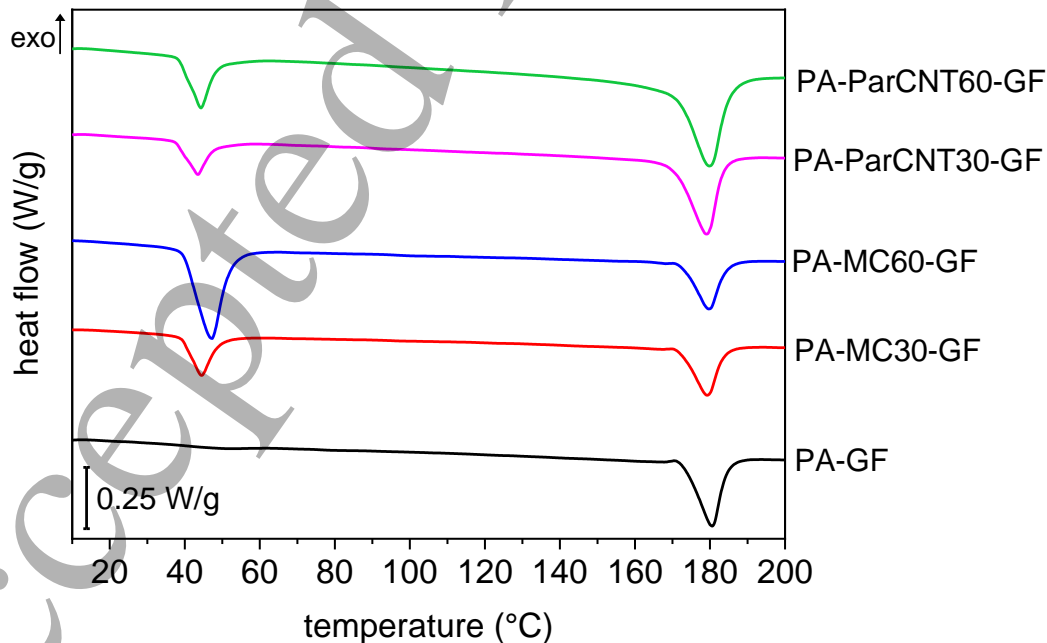
Figure 9. DSC thermograms (first heating scan) of the laminates PA/PCM/GF (10 °C/min; N 2 ) (data from [146]).
