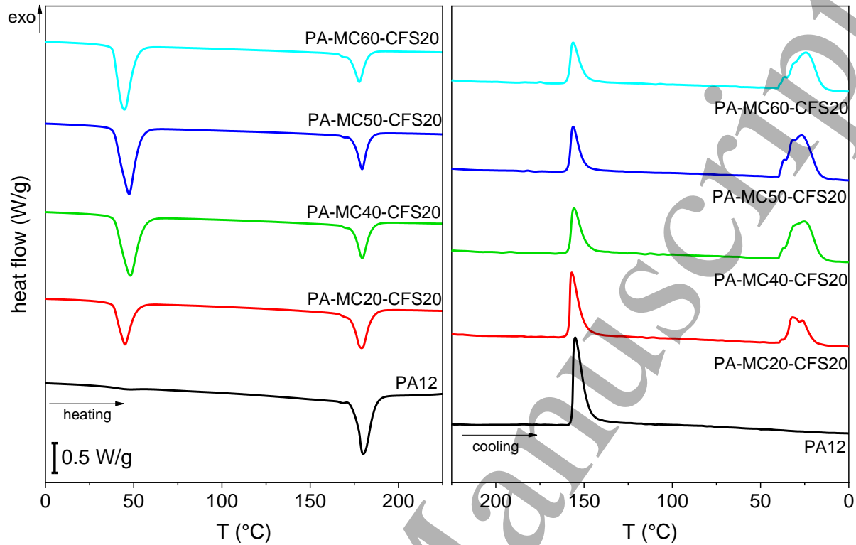
Figure 11. DSC thermograms (heating scan and cooling scan) of the samples PA-MC x -CFS20 (10 °C/min; N 2 flow = 100 ml/min) (data from [148]).
