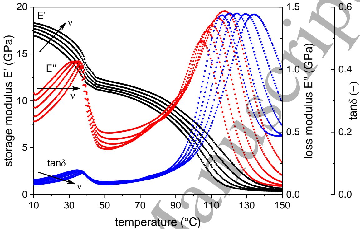
Figure 22. Representative DMA multifrequency thermograms of the sample EL-MC30-CF (single cantilever; 0.3-1-3-10-30 Hz; 0.3 °C/min) (adapted from [158] and [159]).
