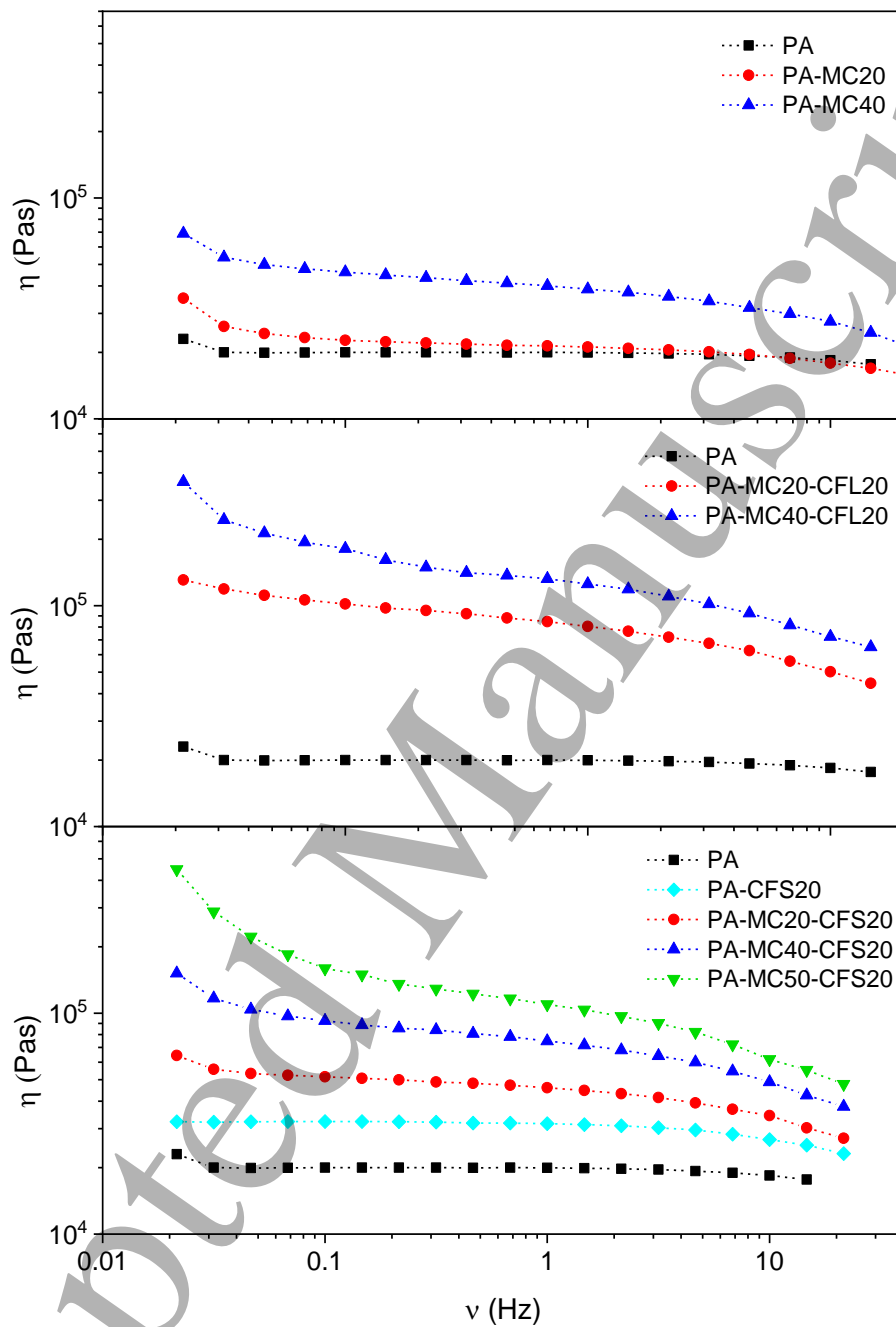
Figure 12. Results of the dynamic rheological test. Values of viscosity as a function of the applied frequency for some representative compositions (parallel plate; gap 1.5 mm; diameter 8 mm; 190 °C; N 2 ) (adapted from [148]).
