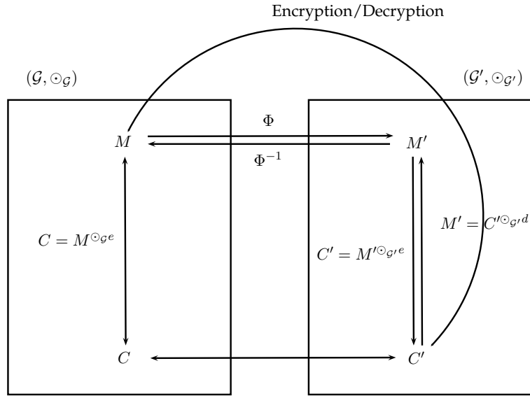
Figure 1: RSA-like scheme based on isomorphism.
