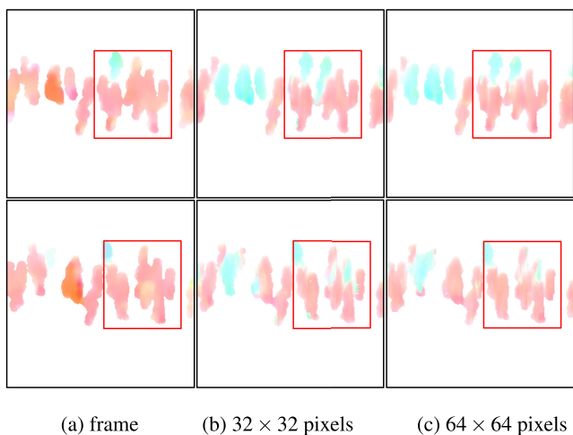
FIGURE 14. Comparison of different sizes of PatchGAN: (b) 32 x 32 pixels and (c) 64 x 64 pixels.
