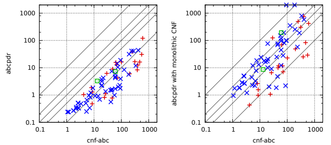
Fig. 16. Comparison of cnf-abc and abcpdr with and without incremental CNF conversion (on selected instances).
