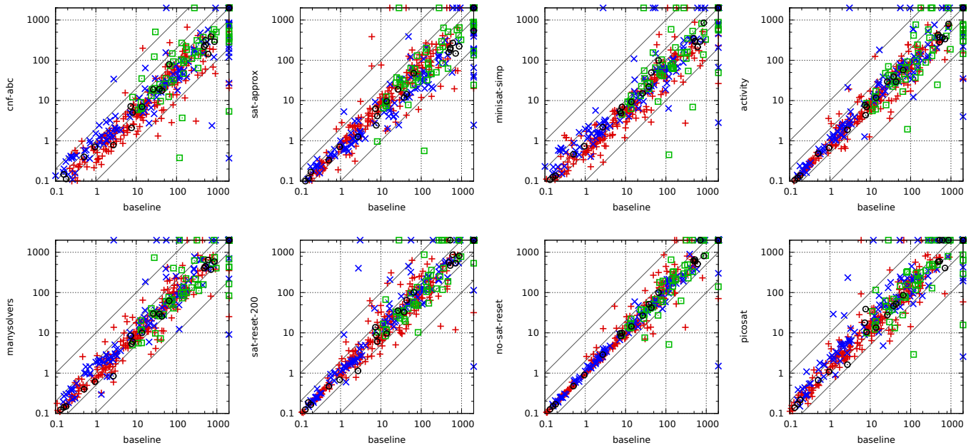
Fig. 13. Detailed comparison of low-level configurations vs the baseline. The baseline is always on the x-axis. Points above the diagonal indicate better performance of the baseline. Points on the borders indicate timeouts (900 s). Different point types denote different benchmark families.
