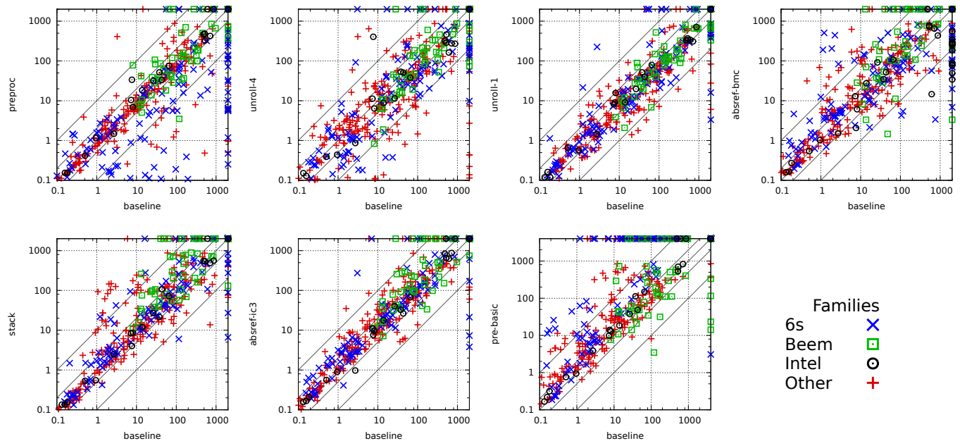
Fig. 11. Detailed comparison of high-level configurations vs the baseline. The baseline is always on the x-axis. Points above the diagonal indicate better performance of the baseline. Points on the borders indicate timeouts (900 s). Different point types denote different benchmark families.
