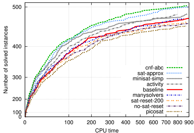
Fig. 12. Survival plots comparing the baseline configuration with configurations changing the low-level parameters.
