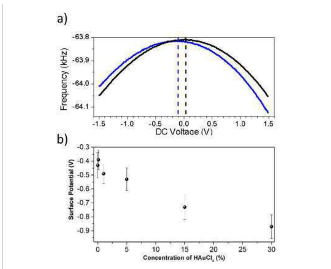
Figure IX.20. (a) Frequency versus voltage curves acquired on SLG on SiO 2 doped with HAuCl 4 for two concentrations [1377]. V_{SP} corresponds to the maximum of the parabolas, marked with dashed vertical lines. (b) The variation of the measured V_{SP} reflects the tuning of E_F upon doping with Au NPs nanoparticles. (Reproduced from [1377], with permission from Elsevier.)
