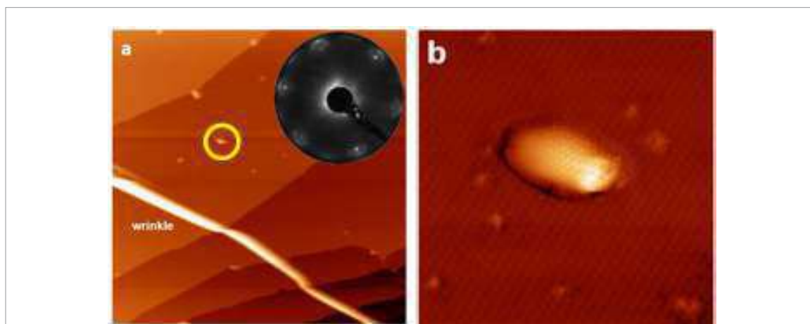
Figure IX.24. (a) STM image of a 200 \times 200 \text{ nm}^2 area of graphene grown on Pt(1 1 1), I = 0.15 \text{ nA} , V = 750 \text{ mV} . A SLG covers the whole surface. In the image a wrinkle/pleat and several nanobubbles, one of them is encircled in yellow, can be seen. The inset shows the characteristic LEED pattern of SLG on Pt(1 1 1). (b) High resolution STM image of a graphene nanobubble ( 20 \times 20 \text{ nm}^2 , I = 0.6 \text{ nA} , V = 310 \text{ mV} ) and few point-like atomic defects with atomic resolution. Figure a is adapted from [1035], with permission from Elsevier.
