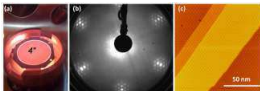
Figure VII.4. (a) 800 °C hot 4 inch wafer in the growth chamber. (b) Low energy electron diffraction (LEED) pattern of h-BN/Rh(1 1 1) at 60 eV kinetic energy. (c) STM image of the same surface with U_t = -1.2 V and I_t = 0.5 nA.
