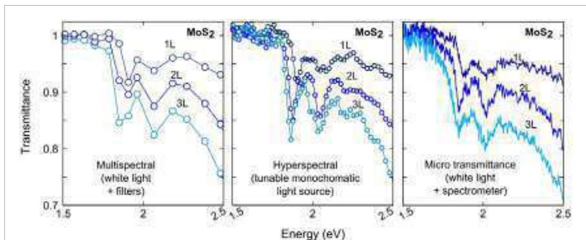
Figure IX.10. Comparison between different methods to measure the optical properties of 1L, 2L, 3L-MoS 2 . In multispectral imaging narrow bandwidth filters (10 nm FWHM) are used to select the wavelength (the wavelength resolution is limited by the number of filters). In hyperspectral imaging, the illumination is provided through a white light source connected to a monochromator (2–3 nm resolution). In micro-transmittance, white light is collected through an optical fiber (acting as a confocal pinhole) and sent to a CCD spectrometer (~1 nm resolution). Adapted from [1436].
