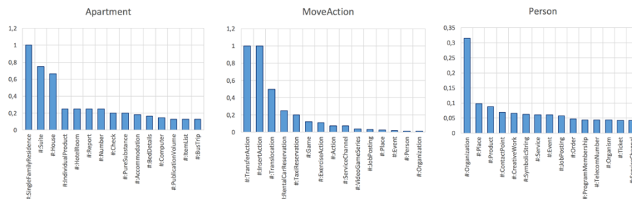
Figure 3. Similarity between different entities in Schema.org and SUMO.
