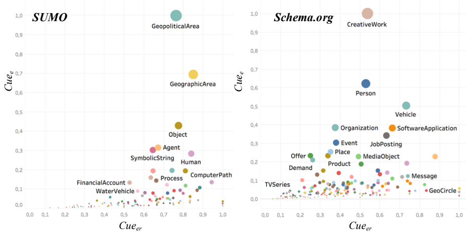
Figure 2. Cue_{er} and Cue_e of SUMO and Schema.org, where the size of the circles denotes the number of properties for that entity.
