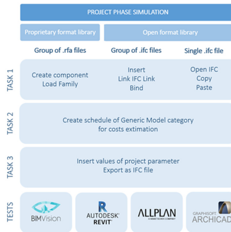
Figure 4: Research method, step 3: diagram of the workflow.
