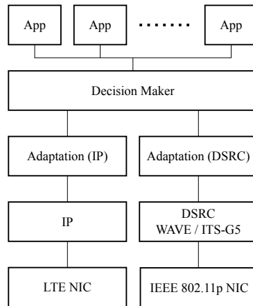
Fig. 13 The heterogeneous networking stack introduced in Veins LTE [21].
