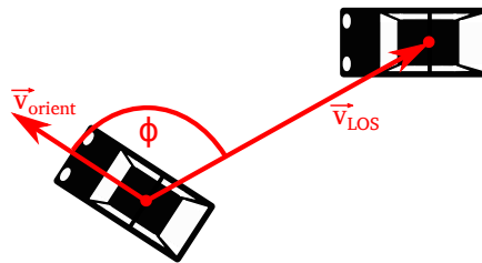
Fig. 7 Dependence of the azimuth angle based on Line of Sight (LOS) and orientation vector.
