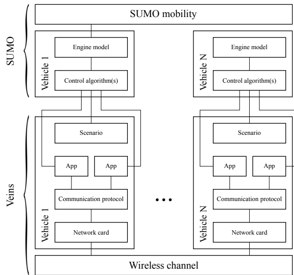
Fig. 11 High-level architecture of PLEXE components.
