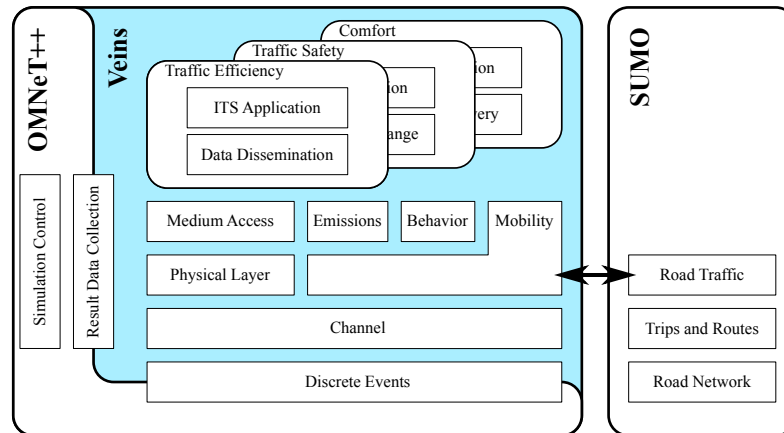
Fig. 1 High-level architecture of Veins.
