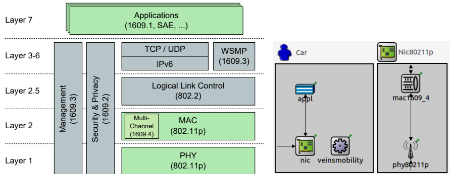
(a) The IEEE Wireless Access in Vehicular Environments (WAVE) family of standards. Layers represented in Veins are colored in green. (b) Layer representation in OMNeT++
