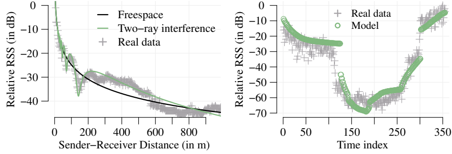
(a) Real-world measurements compared to the free-space model and the two-ray interference model based on [52] (b) Real-world measurements compared to the obstacle model in 2 based on [55]
