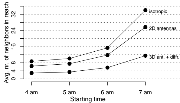
Fig. 9 Average number of neighbors in reach when simulating the LuST scenario with and without 2D antenna patterns as well as 3D antenna patterns (including diffraction effects) [8].
