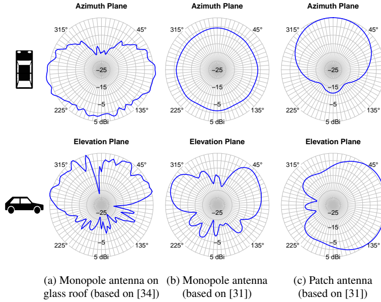
Fig. 5 Azimuth and elevation planes of exemplary vehicular antenna patterns. The gain is given in dBi.
