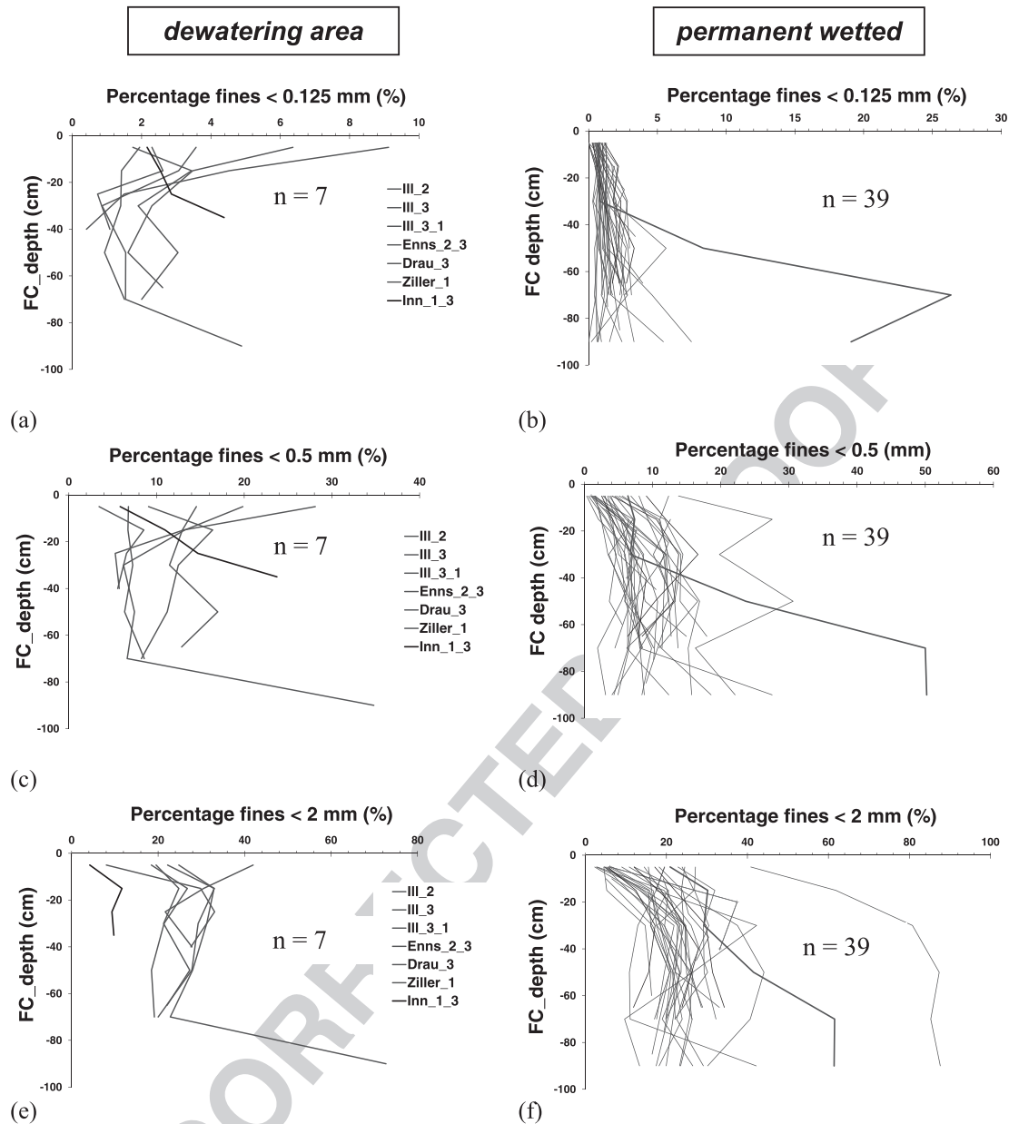
Figure 7. Variability in fine sediment infiltration concerning freeze-core depth in dewatering and permanent wetted areas of hydropeaking reaches in Austria using thresholds d < 0.125 mm (a, b), d < 0.5 mm (c, d) and d < 2 mm (e, f).
