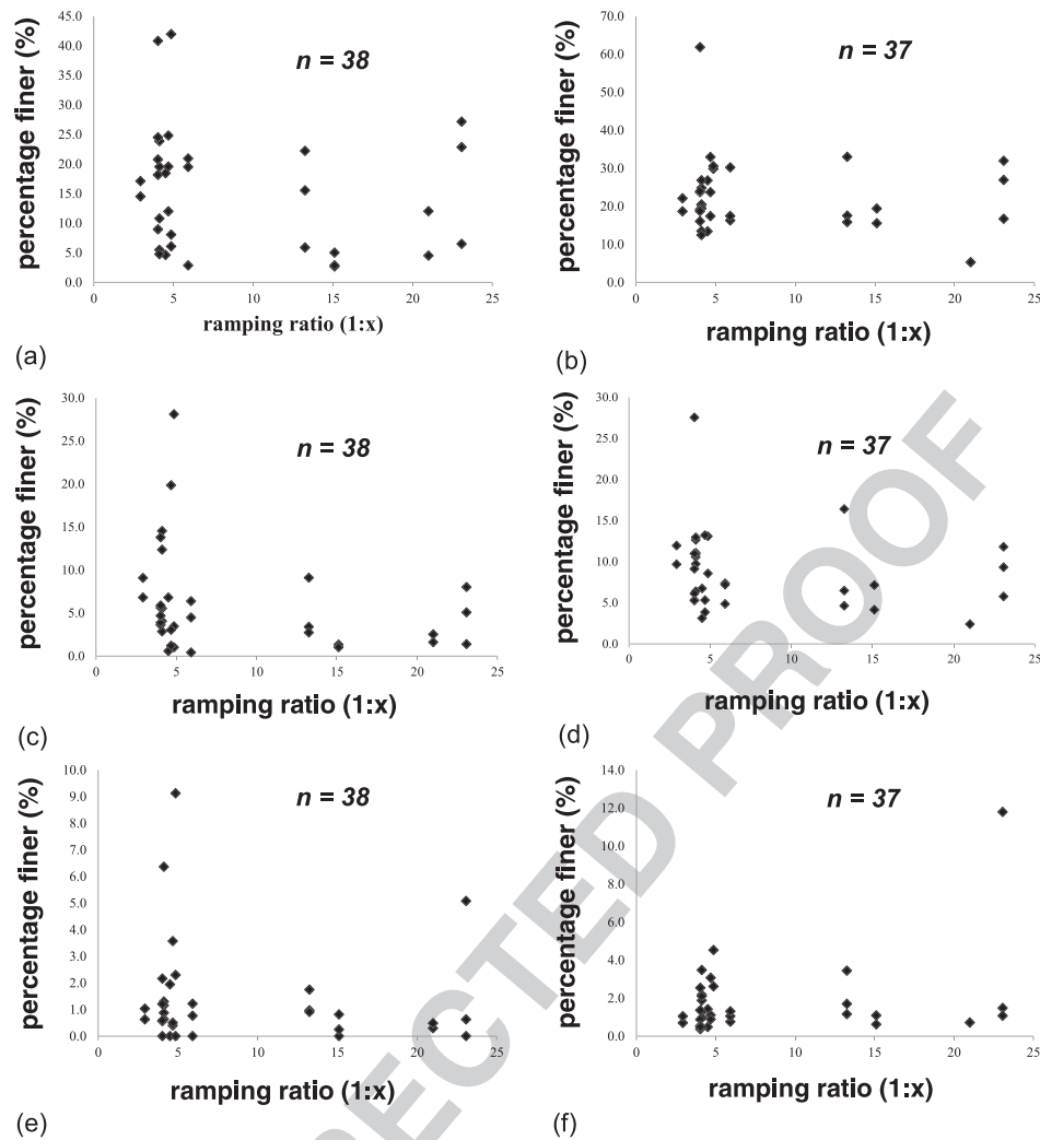
Figure 8. Fine sediment infiltration for truncated samples at 31.5 mm. Different thresholds for quantification have been applied (a,b < 2 mm; c,d < 0.5 mm; e,f < 0.125 mm) as well as the analysis of different vertical layers; Samples (a), (c) and (e) = 0–10 cm (surface layer); Samples (b), (d) and (f) = 10–20 cm (subsurface layer);
