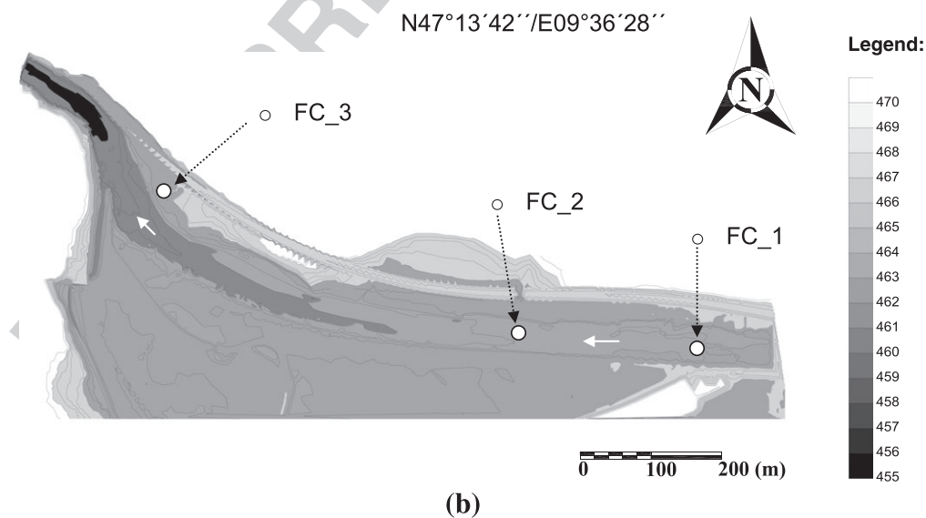
Figure 2. (a) Digital terrain model of the study reach Buchs (Alpenrhein River). Points of stratified (cross-sectional based) freeze-core samples in bar and riffle habitats are highlighted (white dots); flow direction indicated by white arrows; c.s. = cross-section; FC = freeze-core. (b) Digital terrain model of the study reach Ill_2 (Ill River). Points of random freeze-core samples in the investigated section are highlighted (white dots); flow direction indicated by white arrows; FC = freeze-core.
