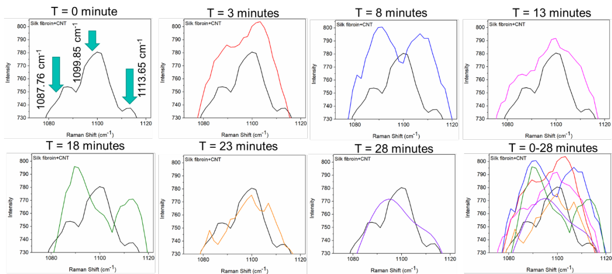
Figure S3: Peak positions range between 1080 \text{cm}^{-1} to 1115 \text{cm}^{-1} of silk fibroin+CNT varies at different time interval from 0 minute to 28 minutes. The spectra obtained at t = 0 minute is used as reference for other panels.
