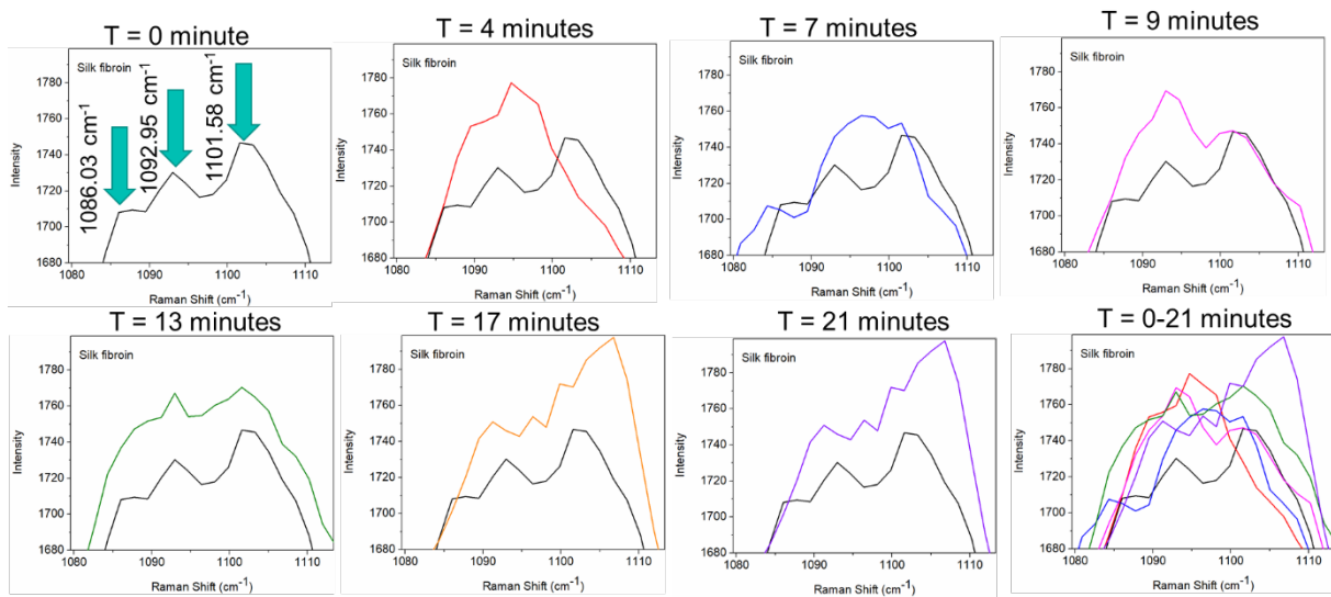
Figure S2: Peak positions range between 1080 cm -1 to 1110 cm -1 of silk fibroin varies at different time interval from 0 minute to 21 minutes. The spectra obtained at t = 0 minute is used as reference for other panels distinctly indicating transformation in the silk fibroin with time.
