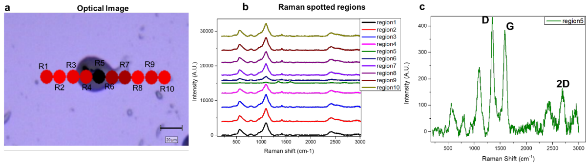
Figure S1: (a) Optical image of RS/CNT marked with different regions R1-R10 over glass substrate. (b) Raman spectrum correspond to the regions marked in panel (a). (c) Region 5 (green colour) is showing the presence of CNT peaks along with Silk fibroin.
