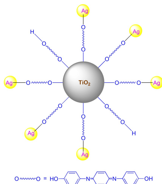
Figure 2. Representation of the \text{TiO}_2/\text{DIOL}/\text{Ag} composite structure. For clarity, only one possible adsorption mode of DIOL onto the \text{TiO}_2 surface is shown; however, adsorption via \pi - \pi interaction of the benzene rings or through the nitrogen lone pair cannot be ruled out.
