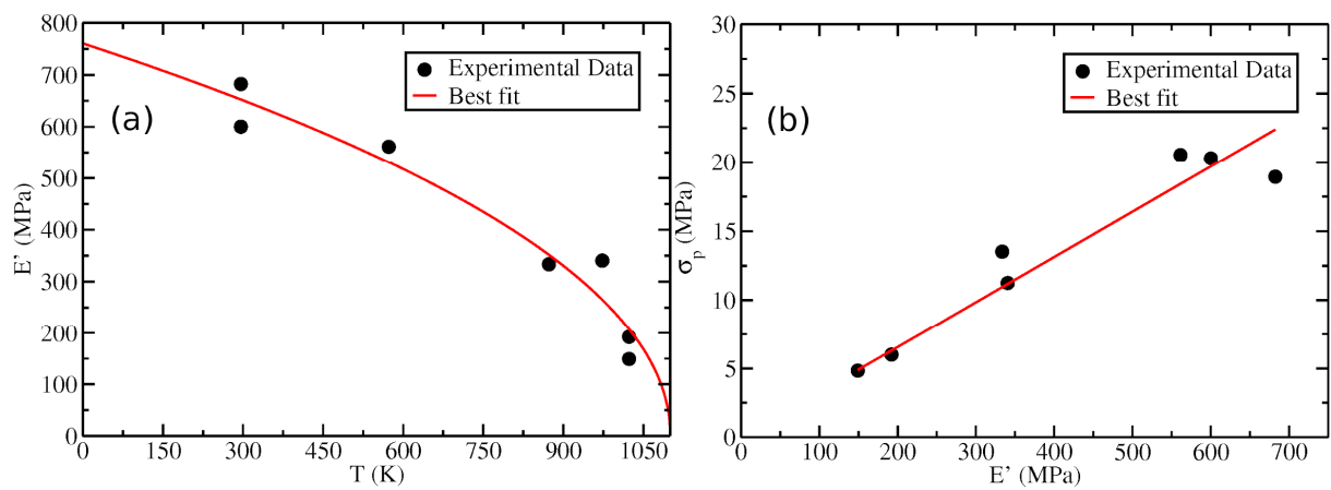
Fig. 6: Best fit curves of (a) effective elastic modulus E' as a function of the temperature T showing an accentuated drop and (b) plateau strength \sigma_p as a function of E' .
