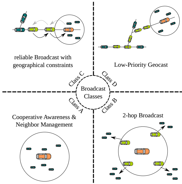
Figure 1. Overview of the four different categories of context aware and class based broadcasting to support a variety of different application domains in vehicular networks.
