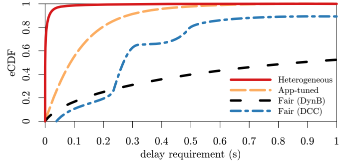
Figure 4. Protocol delay performance as shown in Figure 3 now adding a curve for the heterogeneous networking approach using IEEE 802.11p and VLC (for detailed results see [67]).
