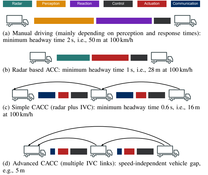
Figure 2. Comparison of vehicle following approaches with their typical achievable performance.
