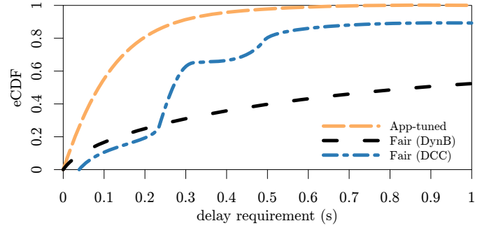
Figure 3. Protocol delay performance (empirical cumulative density function of packets meeting the delay requirement) studying ETSI ITS-G5 DCC, DynB, as well as an app-tuned approach using platooning optimized transmit power and time slotting (figure inspired to [48], for detailed results see the original paper).
