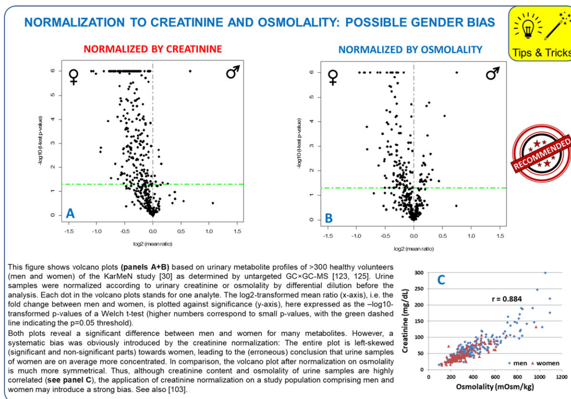
Box 11. Normalization of nutrimetabolomic data: possible gender bias.
