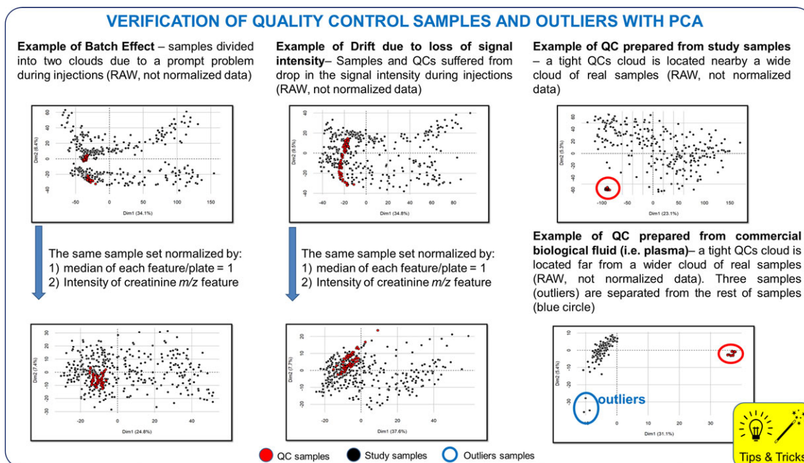
Box 13. Use of PCA for verification of data quality. PCA visualization of study samples and QC samples affected by: batch effect (left site), drift due to loss of intensity (middle), presence of outliers (right site).
