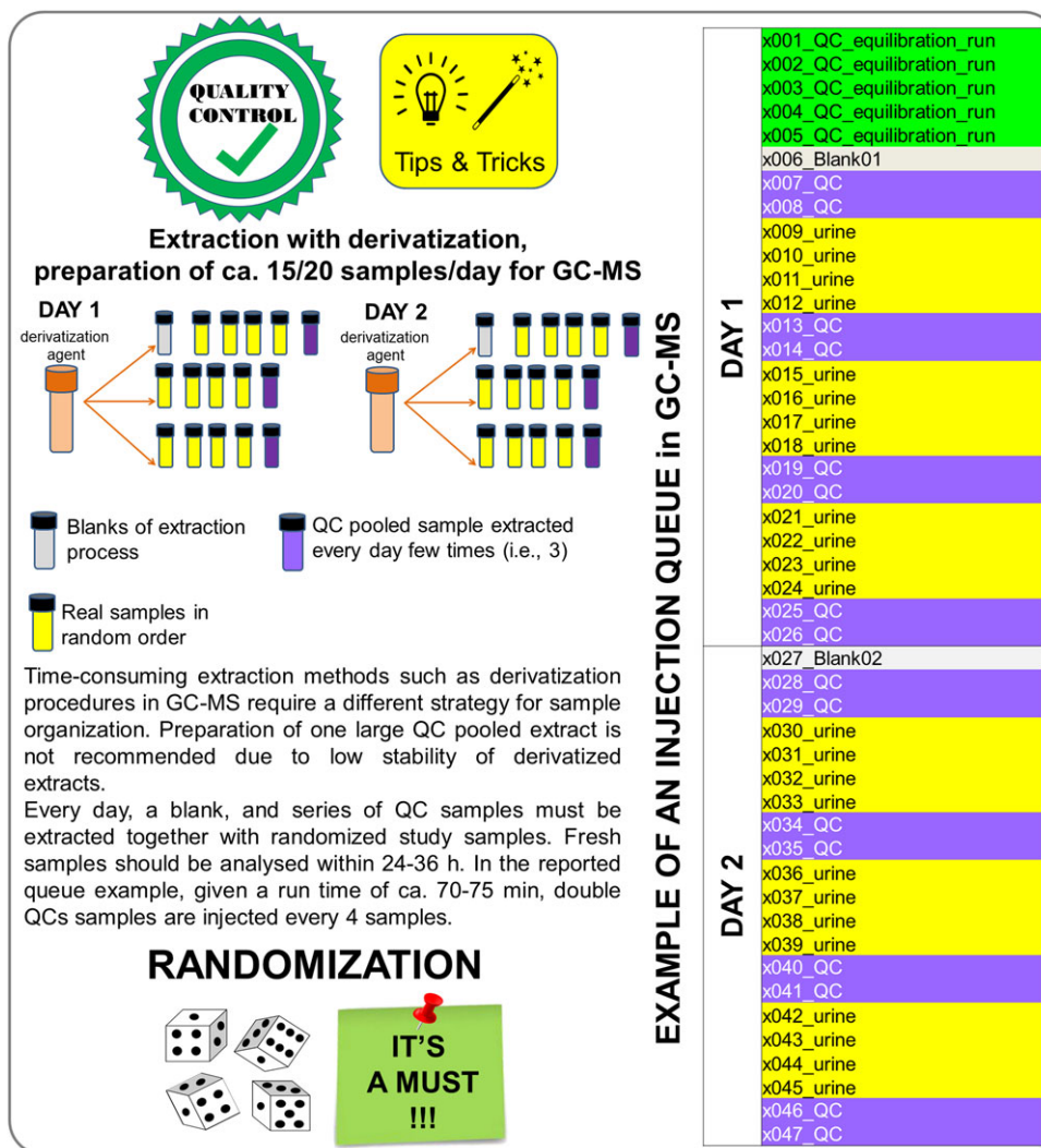
Box 10. GC-MS analysis: preparation of QC samples and injection queue.
