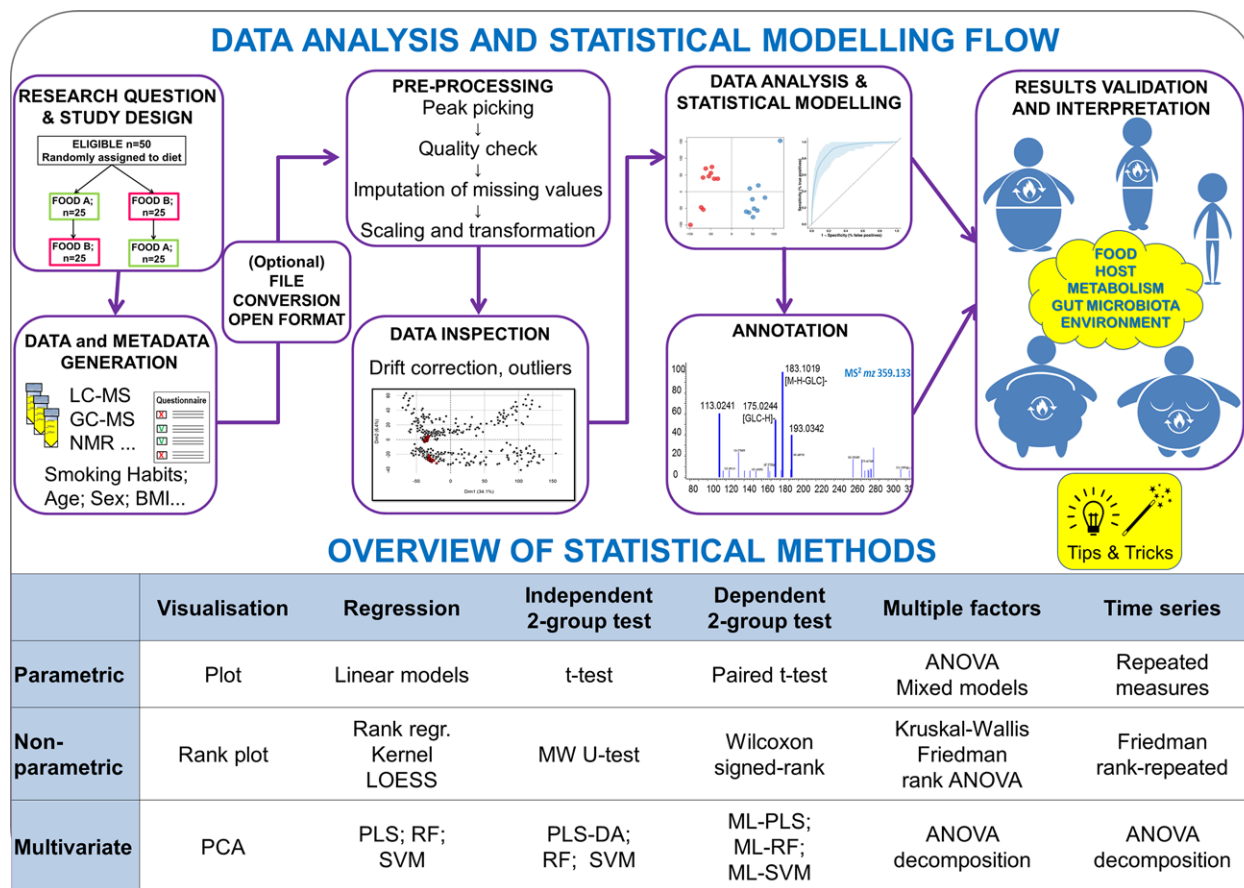
Box 12. General modelling flow for data analysis and selection of statistical methods.
