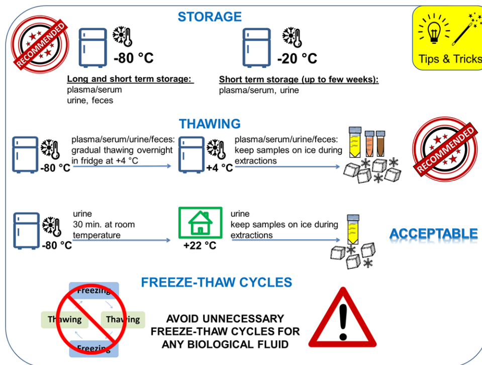
Box 8. Different storage and thawing conditions for biospecimens.
