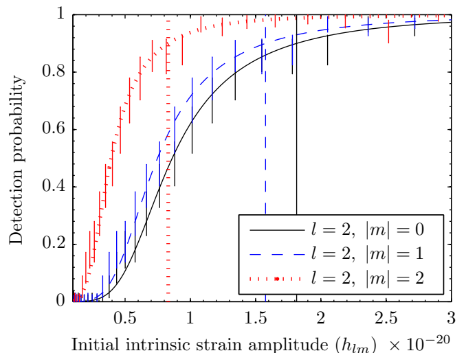
FIG. 5: Detection probabilities for software injections of ring-downs described by Eq. (10) and with parameters drawn from the prior distributions used in the search and described in Sec. IV A. Efficiencies are computed by counting the number of detections in discrete bins in amplitude. The three different curves correspond to the different harmonics (values of |m| ). The long vertical lines indicate the 90% detection efficiencies for the different harmonics, whose numerical values are given in the text. The shorter vertical bars indicate 90% binomial confidence intervals in the estimate of the detection probability in each amplitude bin. The color-coding and line-style convention is the same as that in Figs. 3 and 4: The l = 2 , |m| = 0 efficiency curve is shown as the solid black line, the dashed curve (blue in the on-line version) shows the l = 2 , |m| = 1 efficiency curve and the l = 2 , |m| = 2 efficiency curve is shown as the dotted curve (red in the on-line version).
