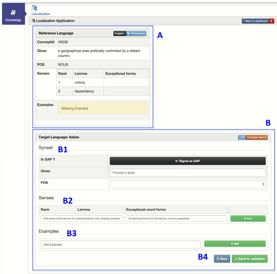
Figure 2: UI design to complete a lexicalization. A corresponds to the source language part. B corresponds to the target language part. B1 corresponds to the gloss and POS of the word. B2 corresponds to the lexicalization of the word. B3 corresponds to the example of the word use. B4 buttons to save or submit the lexicalisation.
