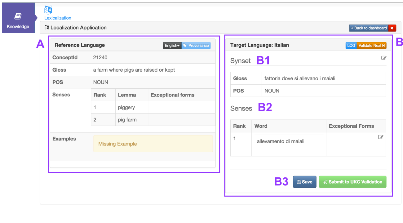
Figure 3: UI design to complete an evaluation. A corresponds to the source language part. B corresponds to the target language. B1 corresponds to the synset. B2 correspond to the senses and B3 are the buttons to save or submit the evaluation over a concept.
