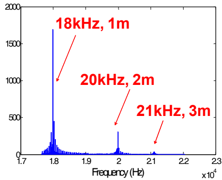
Figure 2. Frequency spectra in proximity of three groups of users
