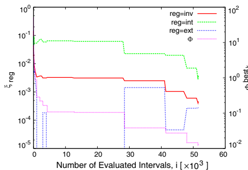
Figure 9. Off-centered homogeneous circular cylinder [ \rho = \frac{\lambda}{4} , \tau = 0.1 , (x_c, y_c) = (-\frac{\lambda}{2}, -\frac{\lambda}{2}) , SNR = 50 dB]. Error Indexes and Fitness Function — Values of the total, internal, and external error indexes and of the fitness function of the best solution retrieved through the IA -based optimization process after the evaluation of each interval.
