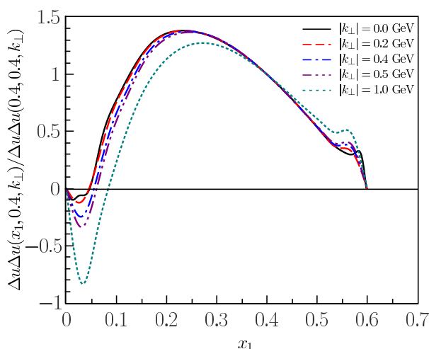
Figure 10. The ratio r_6 , eq. (3.10), for five values of k_\perp .
