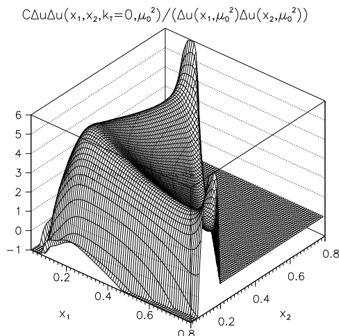
Figure 6. The ratio eq. (3.7) at the hadronic scale.
