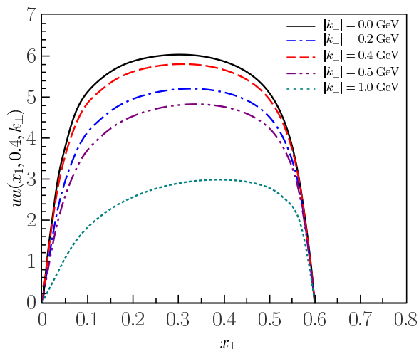
Figure 7. The unpolarized dPDF, eq. (2.24), evaluated at x_2 = 0.4 and at five values of k_\perp .
