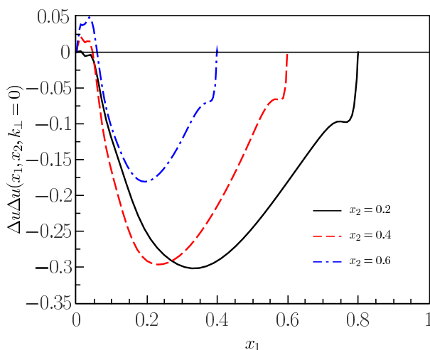
Figure 2. The same as in figure 1, but for the spin-dependent dPDF eq. (2.25).
