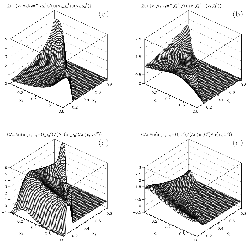
Figure 11. a) The ratio eq. (3.6) at the hadronic scale; b) the same quantity at a scale Q^2 = 10 \text{ GeV}^2 ; c) the ratio eq. (3.7) at the hadronic scale; d) this last quantity at a scale Q^2 = 10 \text{ GeV}^2 . The vertical scale of panels (b) and (d) is reduced by a factor of 2 with respect to panels (a) and (c), respectively.
