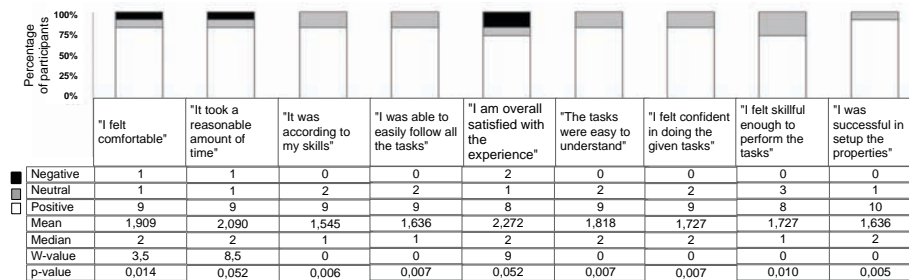
Figure 9: Survey results for questions regarding the overall experience of software developers.
