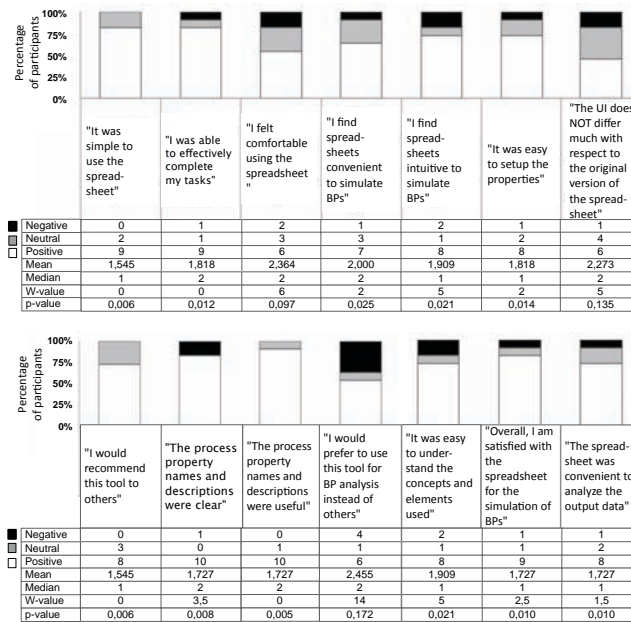
Figure 12: Survey results regarding the use of spreadsheets for BP analysis.
