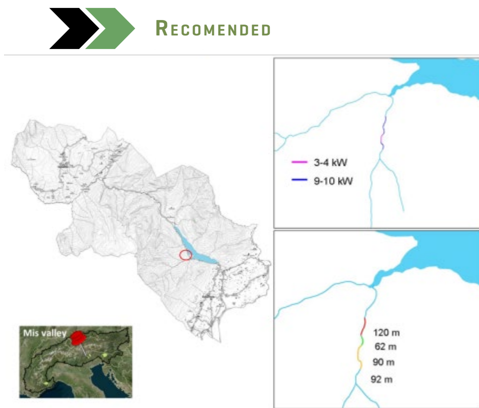
Figure 5.2.5: Map showing the hydropower potential of a stream near Mis lake [Source: Regione Veneto and EURAC]
