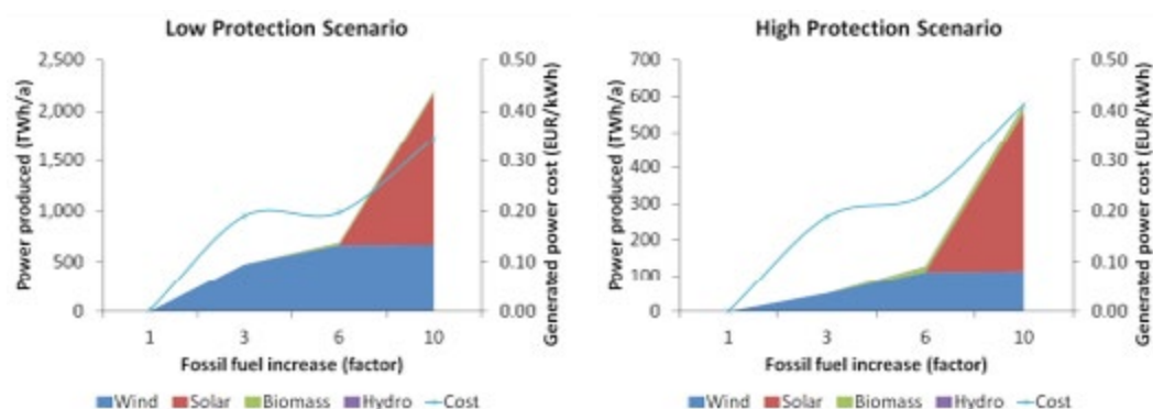
Figure 5.1.7: Potential and cost of renewable energy production in the Alps. [Source: IIASA]
