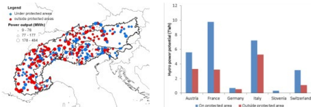
Figure 5.1.5: Optimal location of hydropower plants in the Alps (left) following a business-as-usual scenario and aggregated power generation by country (right). [Source: IIASA]
