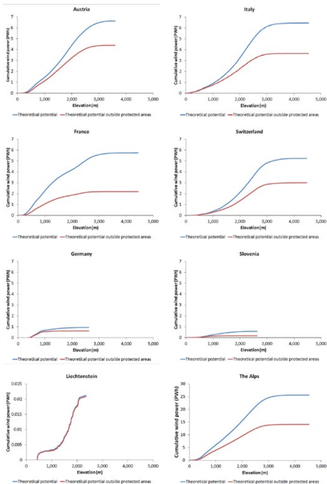
Figure 5.1.2: Profile of the theoretical cumulative wind power potential with regard to elevation for the countries of the Alpine Space and the Alps as a whole. [Source: IIASA]
