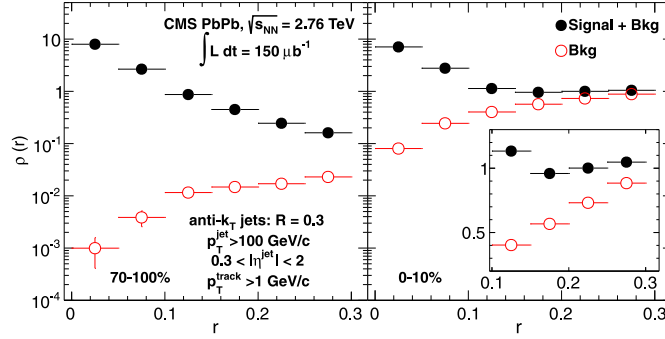
Fig. 1. (Color online.) Differential jet shapes obtained from the jet cone before background subtraction (filled circles), and from the “ \eta -reflected” background cone (open circles), as a function of the distance from the jet axis in two PbPb centrality intervals: 70–100% (left) and 0–10% (right). The measurements use inclusive jets with p_T^{\text{jet}} > 100 GeV/c and 0.3 < |\eta| < 2 , and charged particles with p_T^{\text{track}} > 1 GeV/c.
