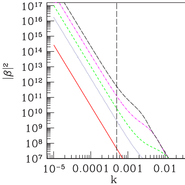
FIG. 1 (color online). The Bogoliubov coefficient |\beta_3(k)|^2 for t_1 = 1 , and t_3 = 2000 , with various values of t_2 . Only the k -values left of the vertical dashed line satisfy kt_3 < 1 . They show clearly a k^{-4} slope and the amplitude is well approximated by (38).
