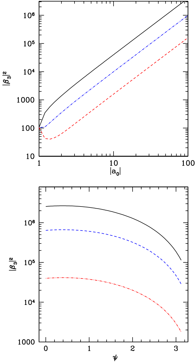
FIG. 2 (color online). In the top panel we show |\beta_3|^2 as a function of \alpha_0 for \alpha_0 and \beta_0 in phase (top, solid, black line), of opposite phase (lowest, dashed, red line) and with a phase difference of 0.8\pi (middle, dot-dashed, blue line). In the bottom panel we show |\beta_3|^2 as a function of the phase difference \psi for |\alpha_0| = 80 (top line) |\alpha_0| = 40 (middle line) and |\alpha_0| = 10 (lowest line). We have chosen z_1 = 0.1 in this plot and the overall vertical normalization is in units of (2z_2/(z_1z_3))^2 .
